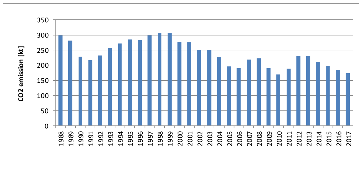
Figure 4.4.4. CO 2 process emission for zinc production in 1988-2017
