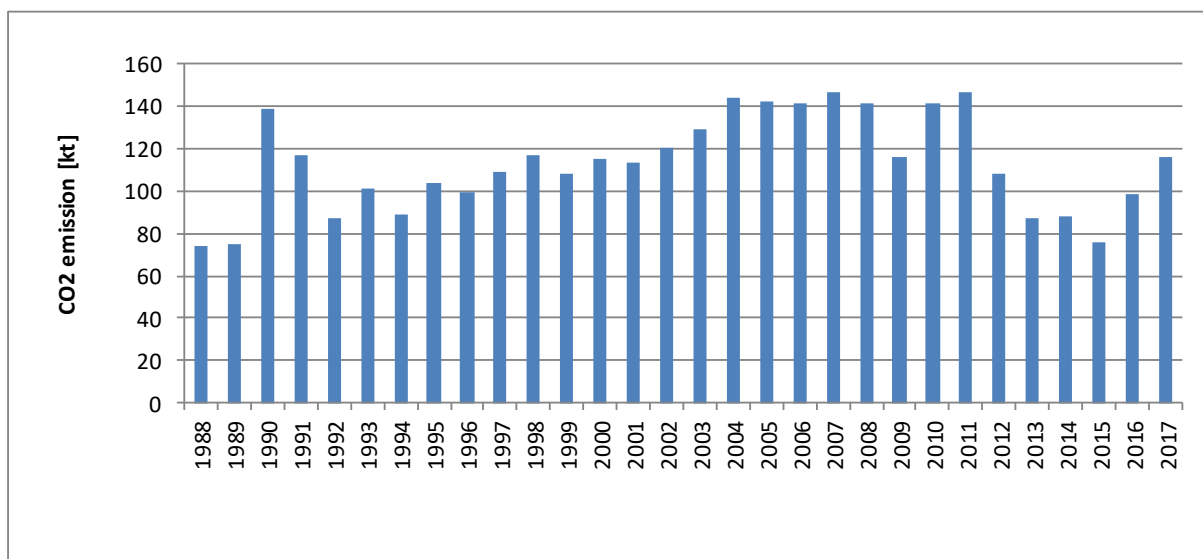
Figure 4.2.10. CO 2 emission values from soda ash use in 2.A.4.b subcategory in the years 1988-2017
