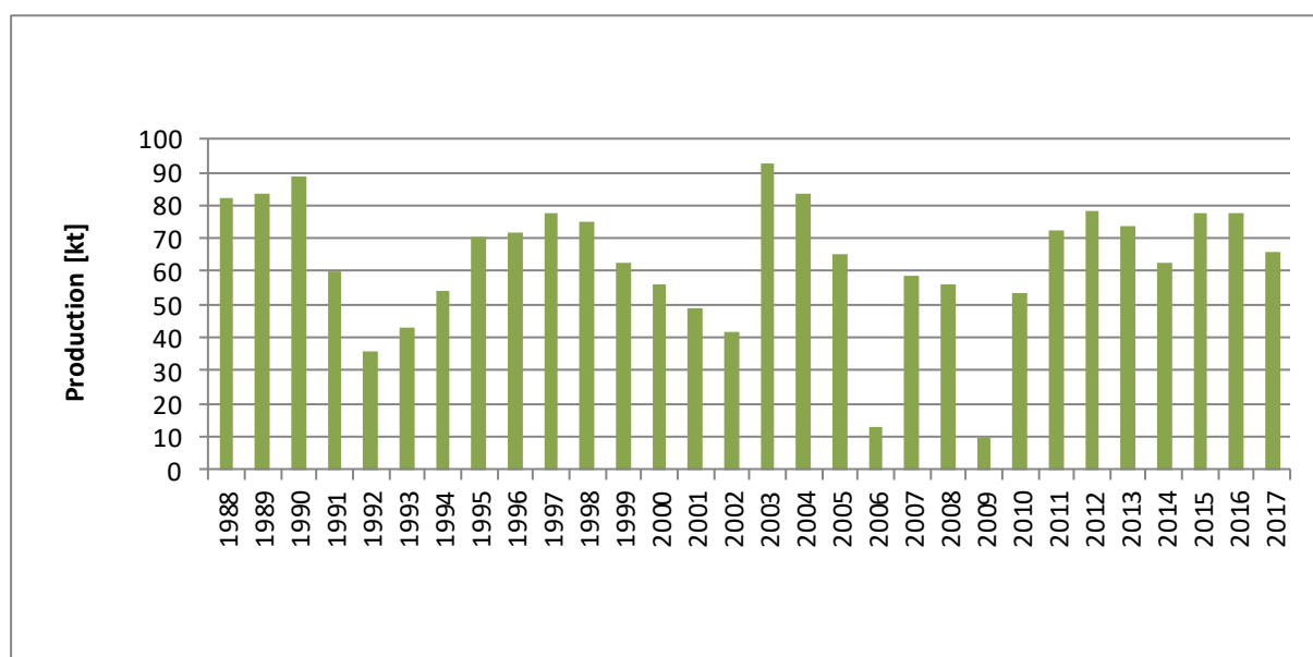
Figure 4.4.2. Production of ferrosilicon in 1988-2017
