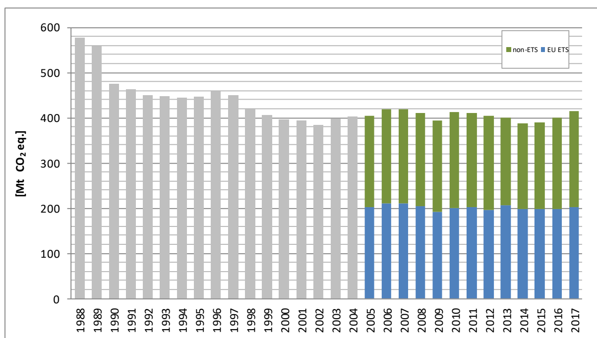
Figure S.2. Trend of aggregated GHGs emissions excluding category 4 for 1988-2017
