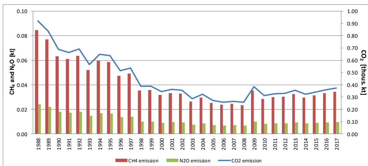
Figure 3.2.8.19. GHG emission in 1988-2017 in subcategory 1.A.4.c.iii
