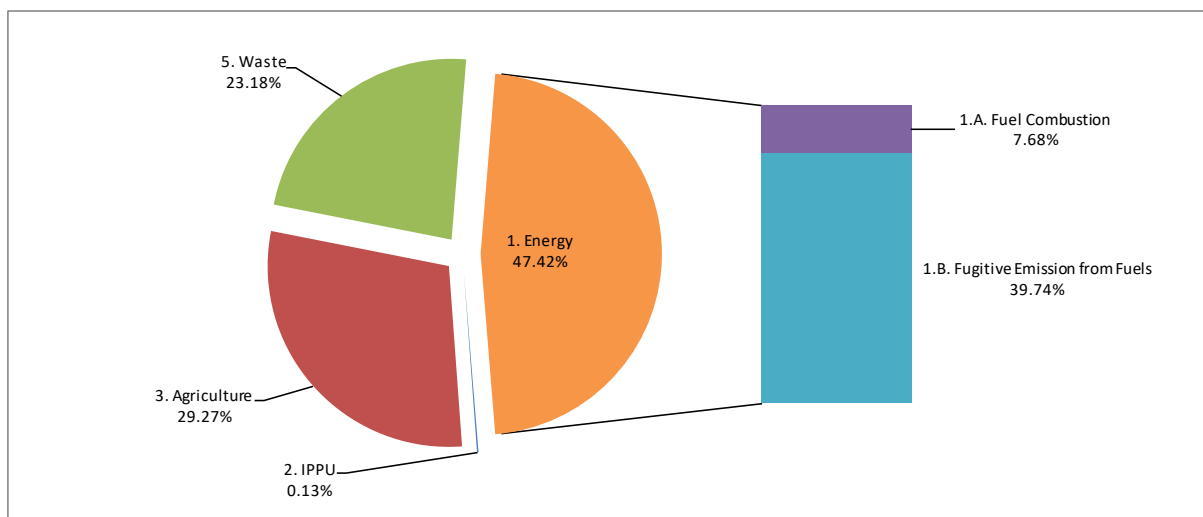
Figure 2.4. Methane emission (excluding category 4) in 2017 by sector
