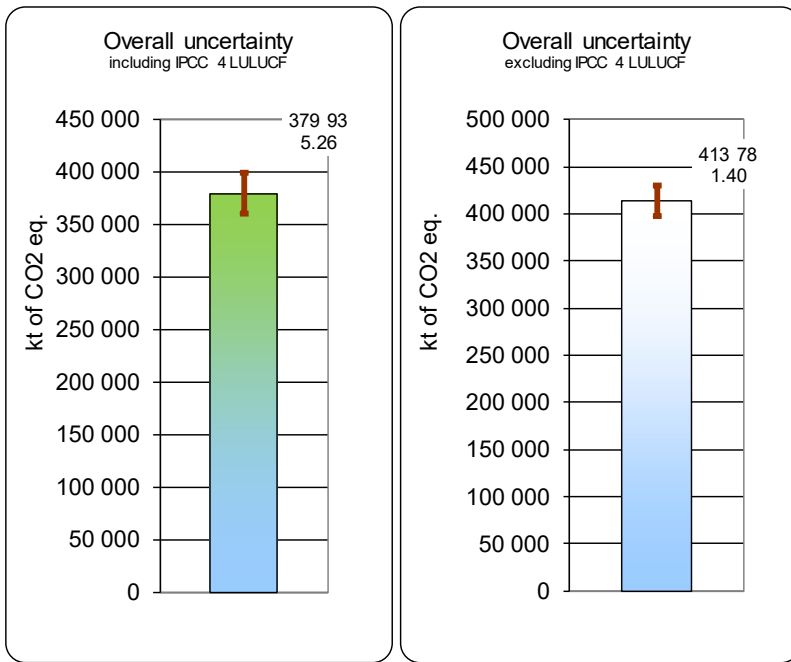
Overall emission results for 2017 including and excluding IPCC 4. LULUCF with uncertainties bars
