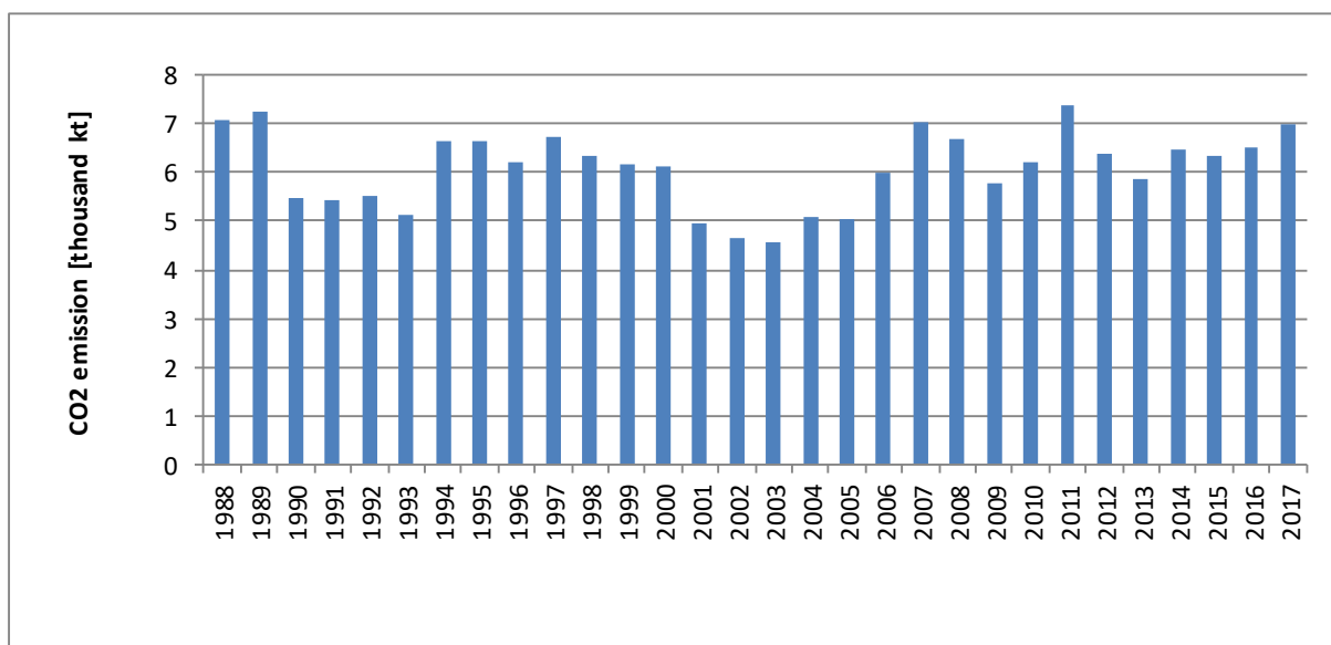
Figure 4.2.3. CO 2 process emission for clinker production in 1988-2017
