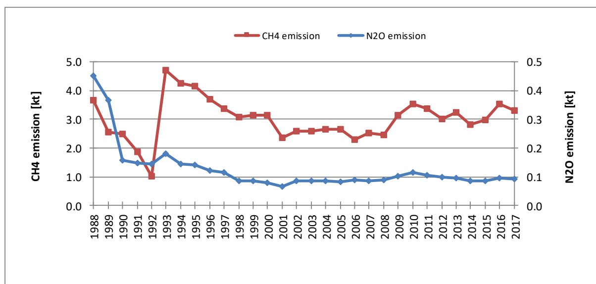
Figure 3.2.9.3. CH 4 and N 2 O emissions for 1.A.4.a category in 1988-2017
