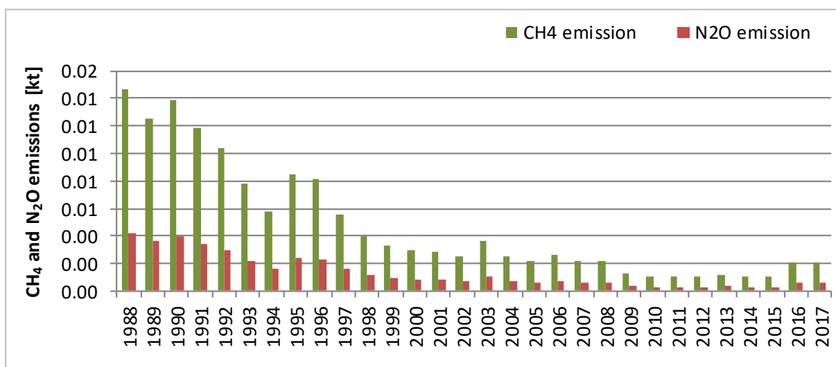
Figure 3.2.8.13. CH 4 and N 2 O emissions for 1.A.3.d category in 1988-2017
