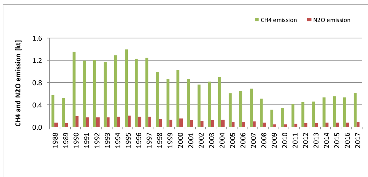
Figure 3.2.7.3. CH 4 and N 2 O emissions for 1.A.2.a category in 1988-2017
