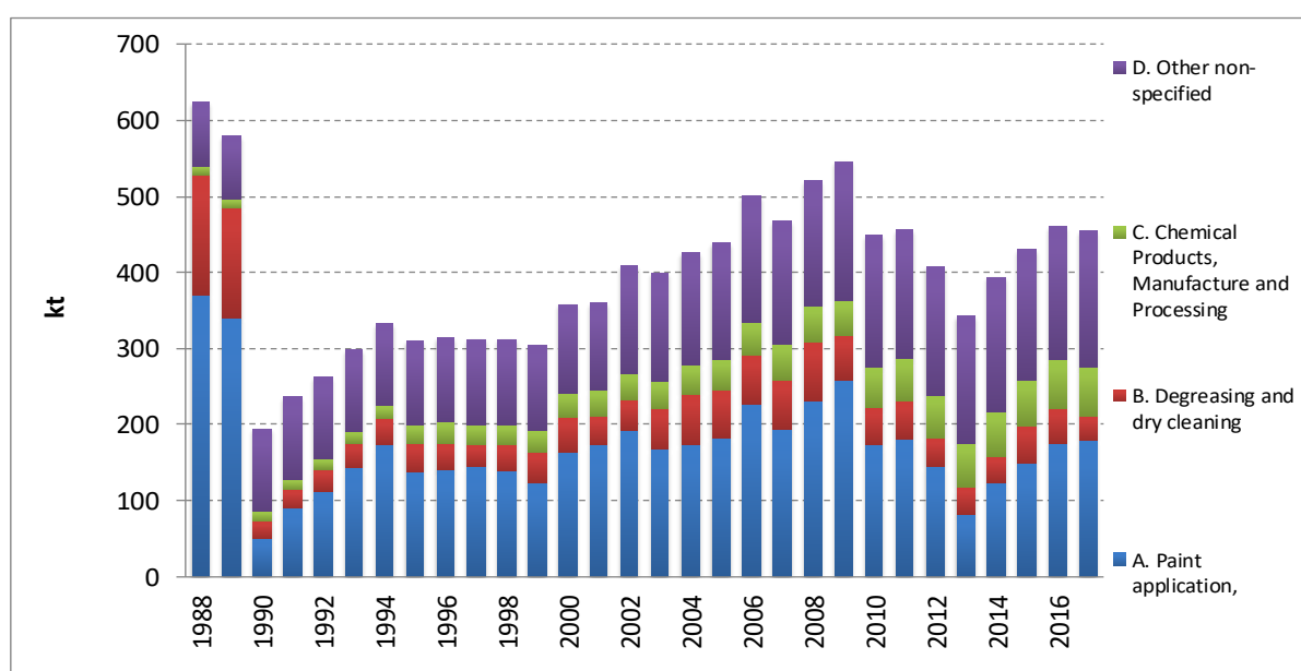
Figure 4.5.5. CO 2 emission from Solvent and Other Product Use sector in 1988-2017
