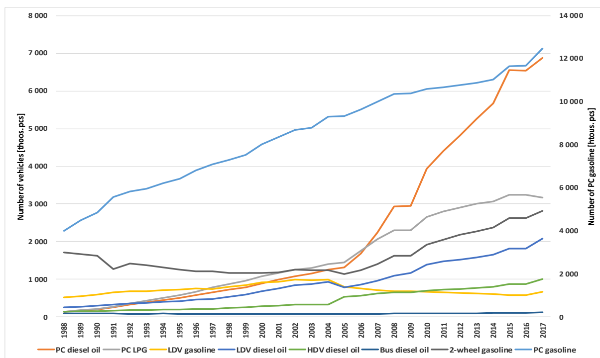
Figure 3.2.8.5. Number of vehicles in years 1988-2017
