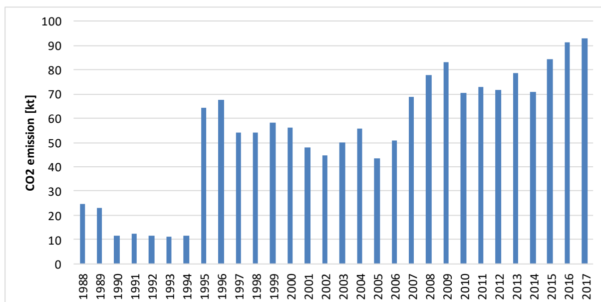
Figure 4.5.3. CO 2 emissions from non-energy use of paraffin waxes in years 1988-2017
