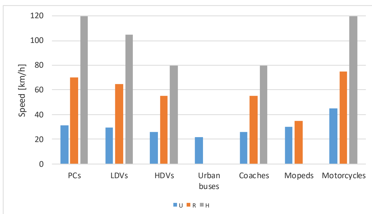
Figure 3.2.8.8. The average speed per road class (urban, rural and highways) in 2017
