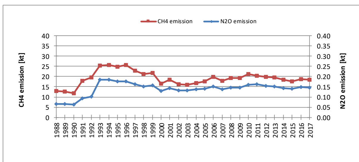
Figure 3.2.9.7. CH 4 and N 2 O emissions in 1.A.4.c.i category in 1988-2017
