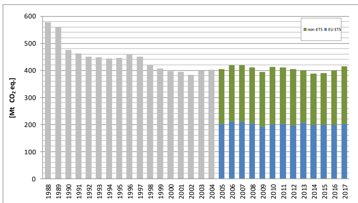
Figure 2.2. Trend of aggregated GHGs emissions (excluding category 4) for 1988–2017
