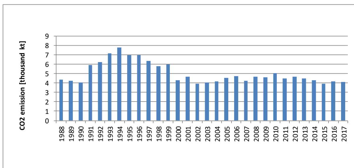
Figure 3.2.9.6. CO 2 emission in 1.A.4.c.i category in 1988-2017
