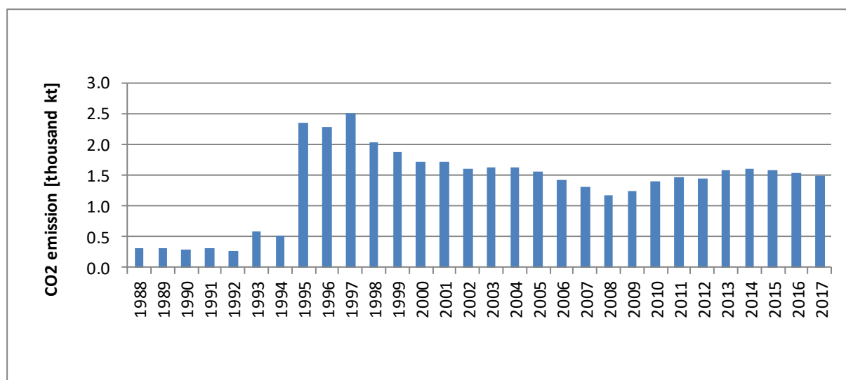
Figure 3.2.7.8. CO 2 emission for 1.A.2.d category in 1988-2017
