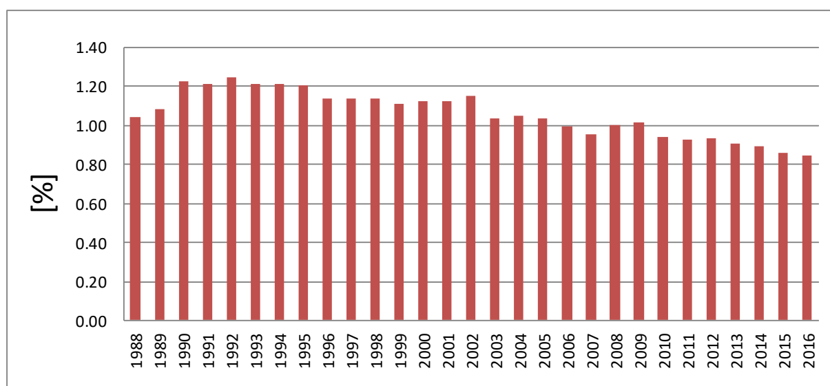
Figure 10.2. Recalculation of CH 4 for entire time series made in CRF 2019 comparing to CRF 2018
