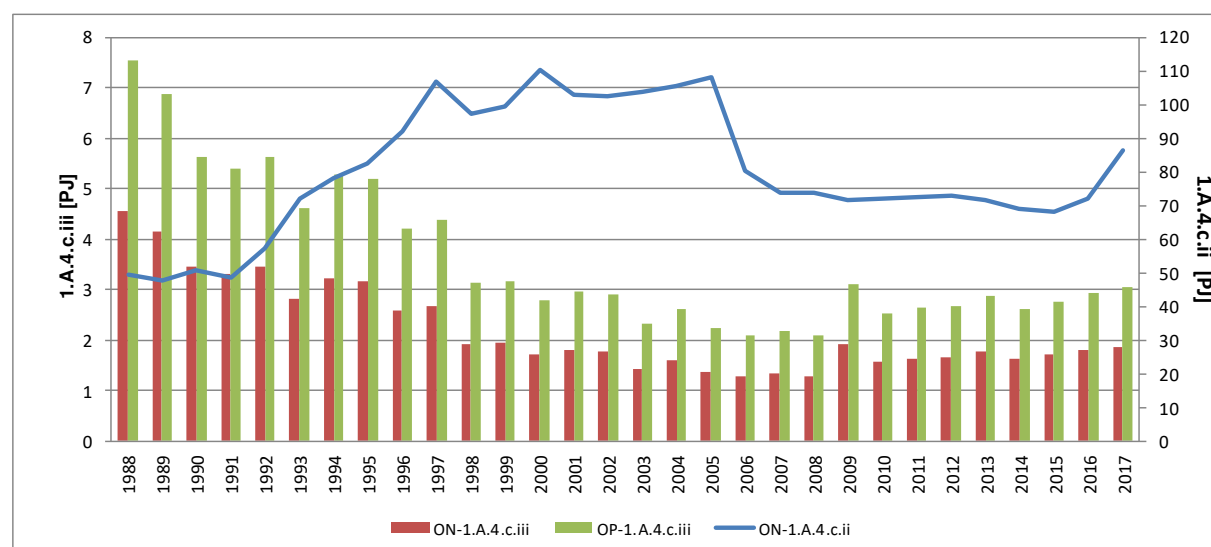
Figure 3.2.8.17. Fuel consumption in 1988-2017 in mobile sources in subcategories other than 1.A.3
