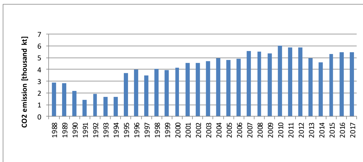
Figure 3.2.6.4. CO 2 emission for 1.A.1.b category in 1988-2017
