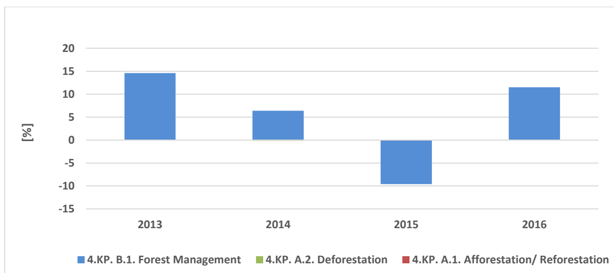
Figure 10.5. Recalculation of CH 4 for 2013-2016 for KP-LULUCF activities made in CRF 2019 comparing to CRF 2018
