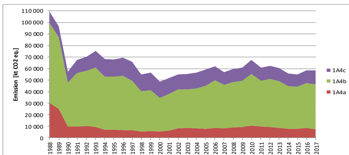
Figure 3.2.9.1. GHG emissions from 1.A.4 Other sectors in years 1988-2017 according to subcategories
