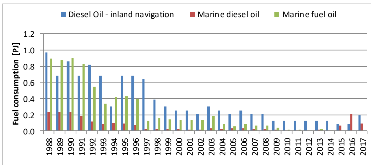
Figure 3.2.8.11. Fuel consumption in 1.A.3.d category for 1988-2017
