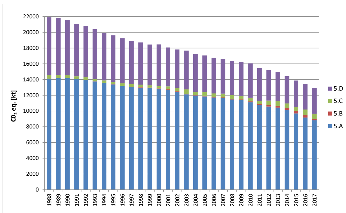
Figure 7.2. GHG emissions from waste sector divided to subsectors in 1988-2017
