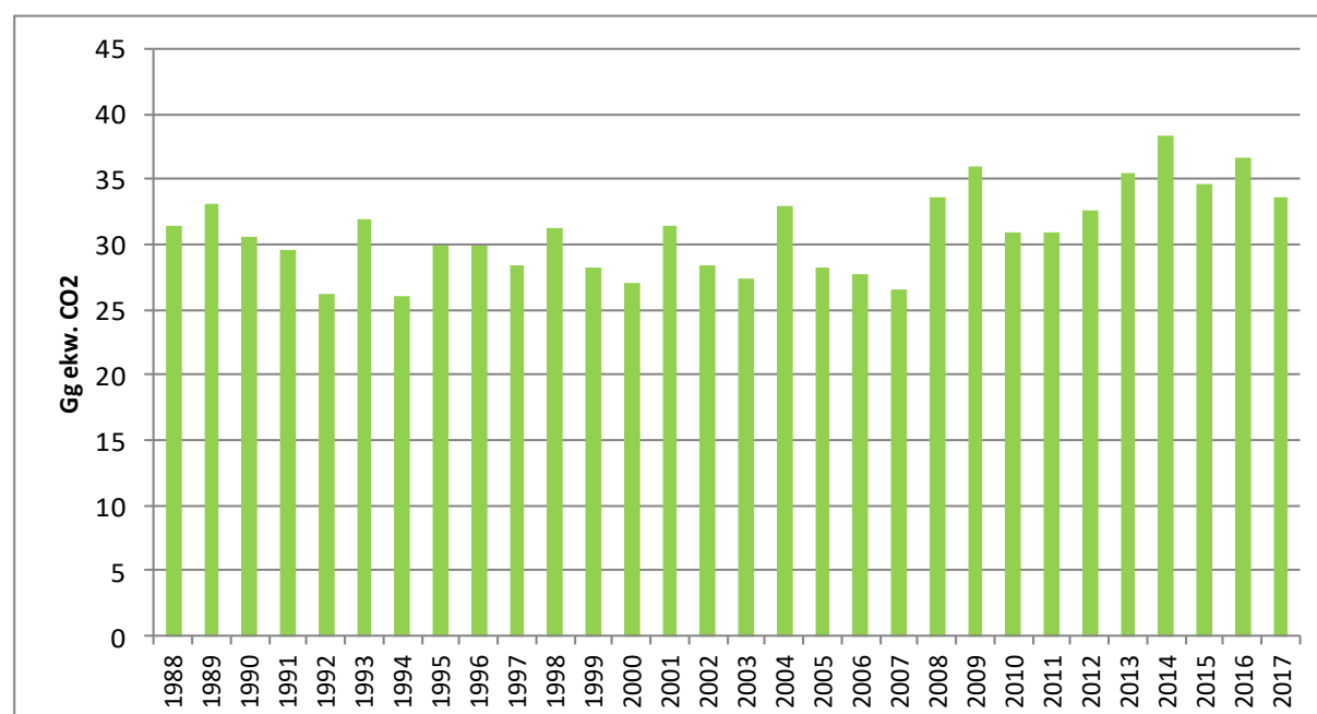
Figure 5.9 CH 4 and N 2 O emissions from field burning of agricultural residues presented as CO 2 equivalent
