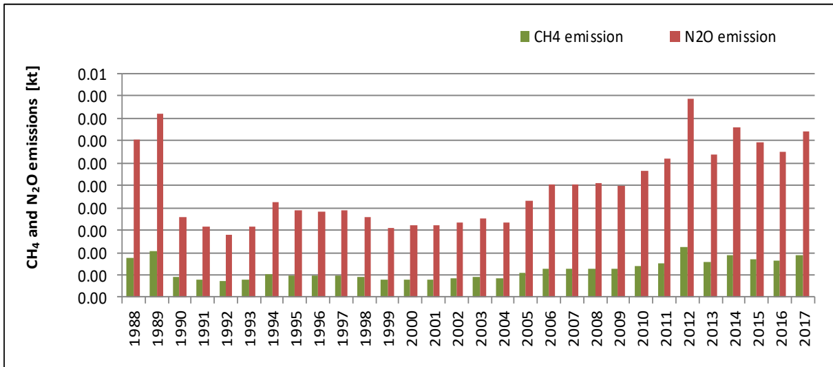
Figure 3.2.8.4. CH 4 and N 2 O emissions for 1.A.3.a category in 1988-2017
