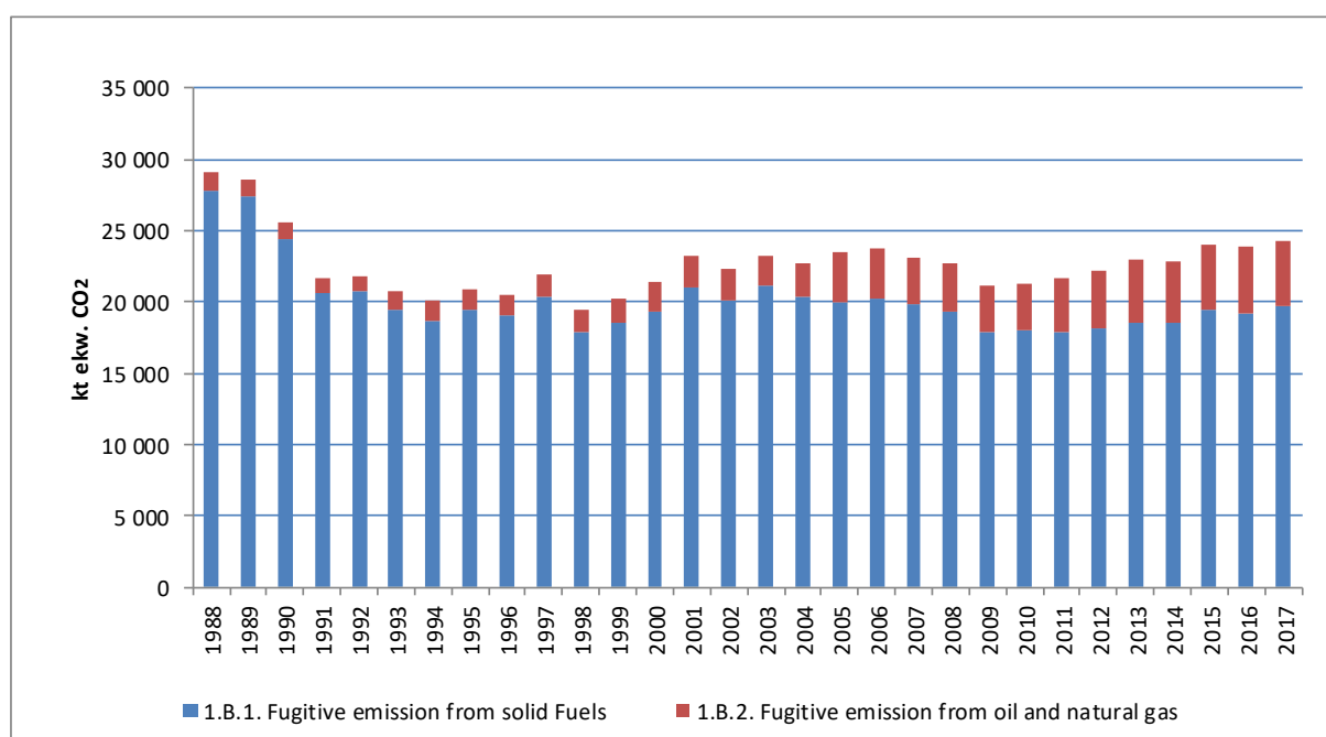
Figure 3.1.4. GHG emissions from 1.B.1 and 1.B.2 subcategories in 1988-2017
