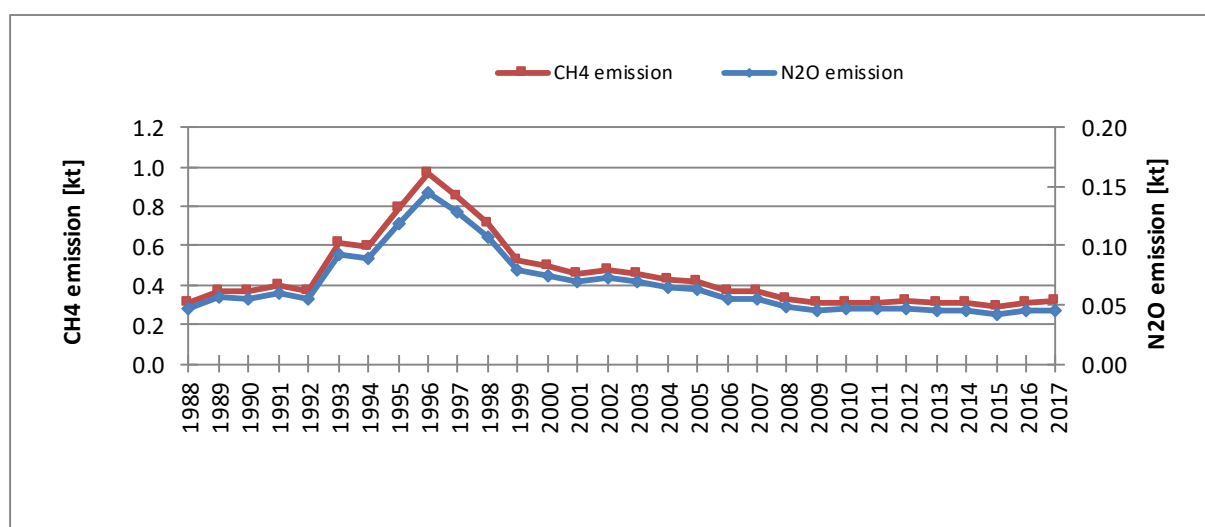
Figure 3.2.7.11. CH 4 and N 2 O emissions for 1.A.2.e category in 1988-2017
