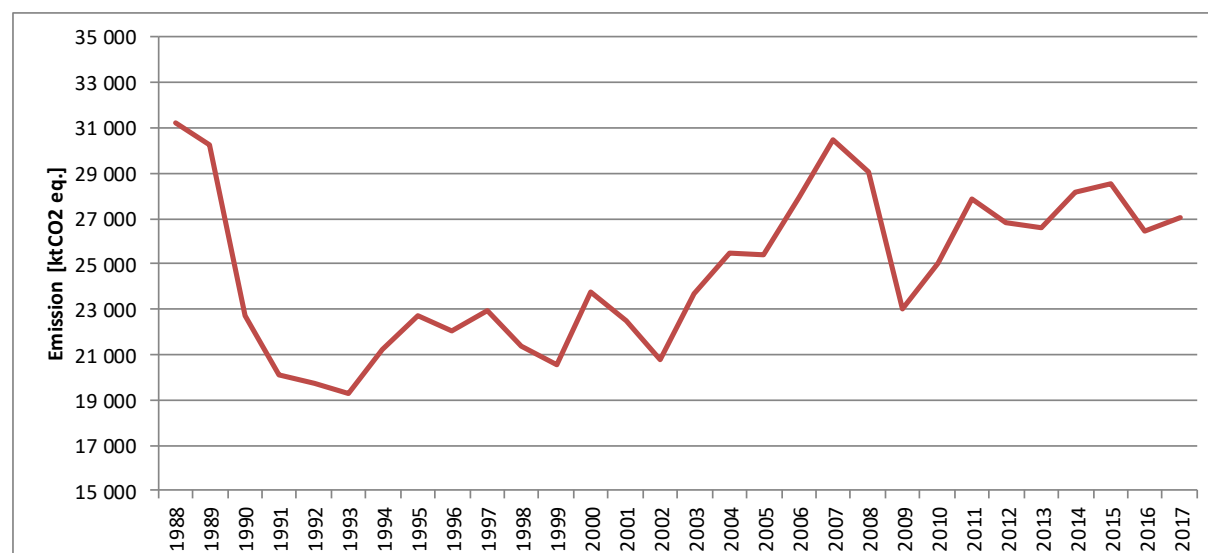
Figure 4.1.1. Emission trend in Industrial processes and product use sector in period 1988-2017
