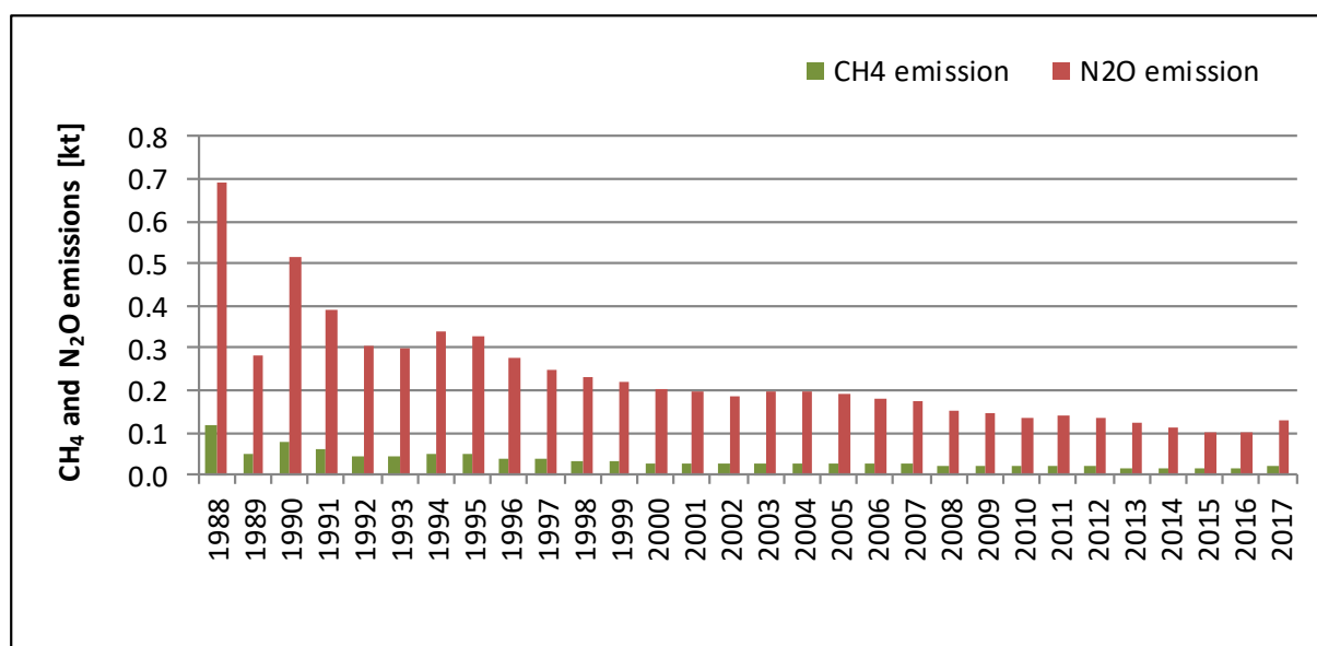
Figure 3.2.8.10. CH 4 and N 2 O emissions for 1.A.3.c category in 1988-2017
