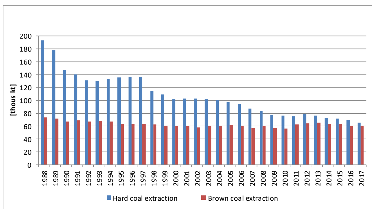
Figure 3.3.1. Hard coal and lignite extraction in 1988-2017
