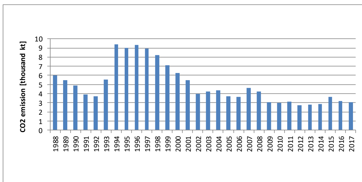
Figure 3.2.6.6. CO 2 emission for 1.A.1.c category in 1988-2017
