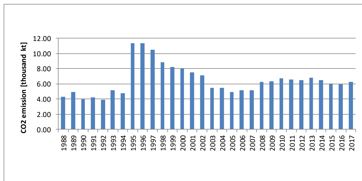
Figure 3.2.7.6. CO 2 emission for 1.A.2.c category in 1988-2017
