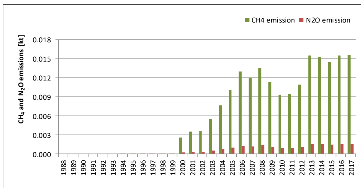
Figure 3.2.16. CH 4 and N 2 O emissions from Pipelines category in 1988-2017
