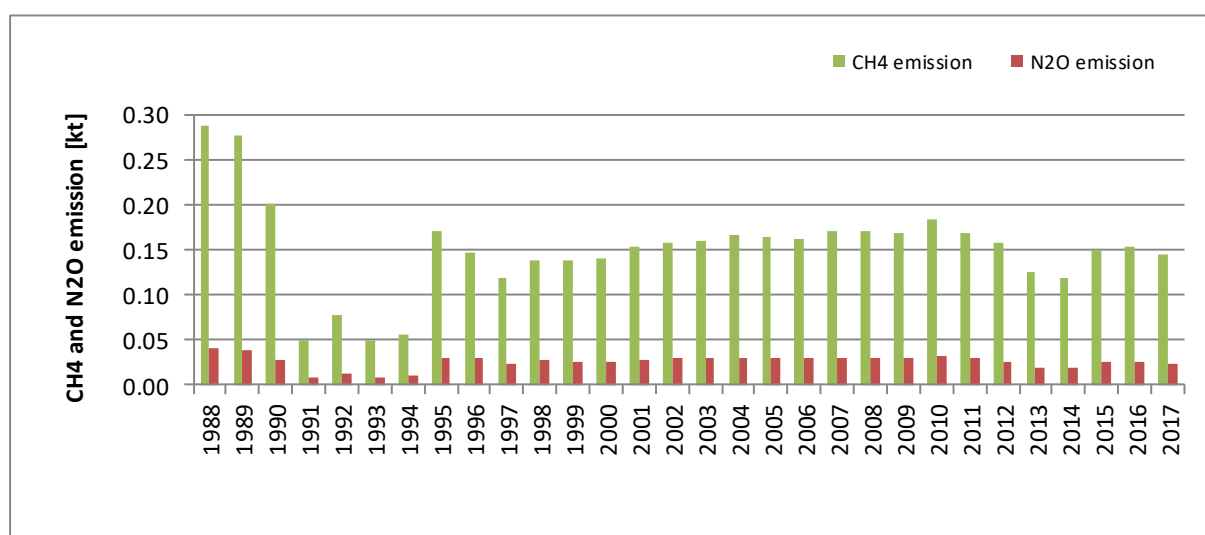
Figure 3.2.6.5. CH 4 and N 2 O emissions for 1.A.1.b category in 1988-2017
