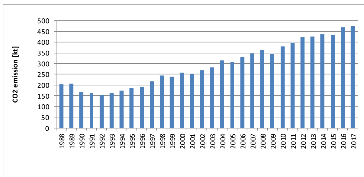
Figure 4.2.7. CO 2 process emission for glass production in 1988-2017
