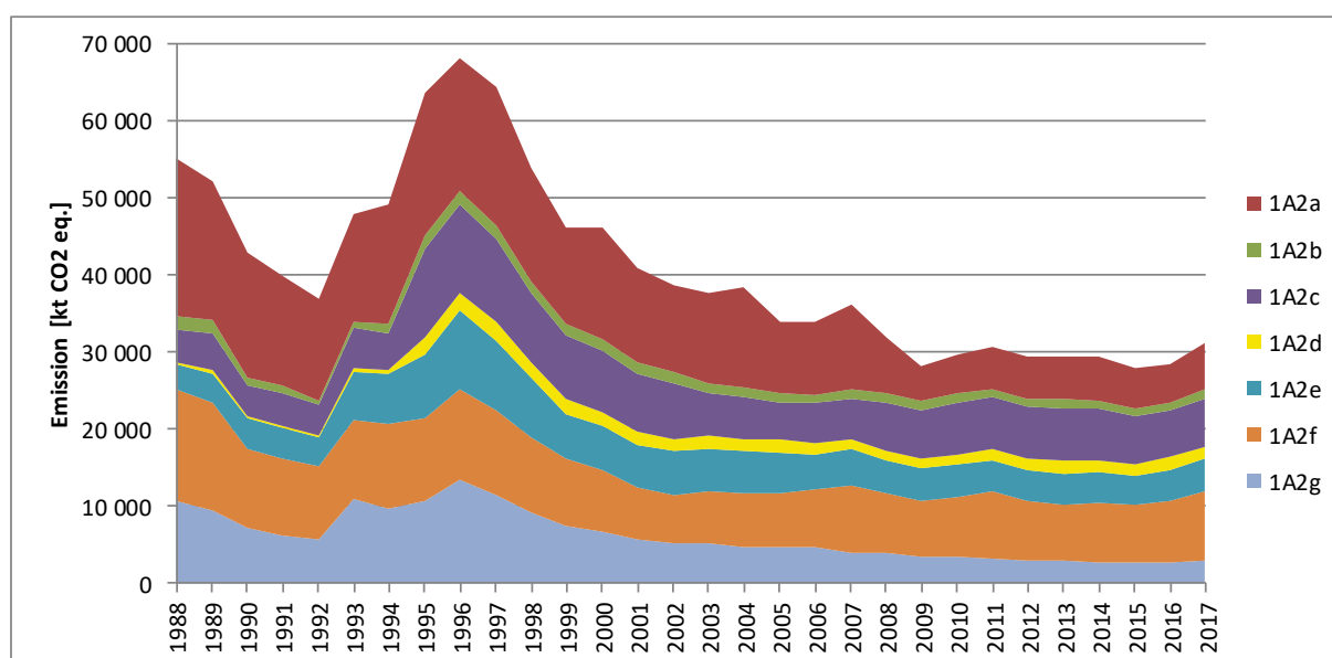
Figure 3.2.7.1. Emissions from Manufacturing Industries and Construction category in years 1988-2017 according to subcategories
