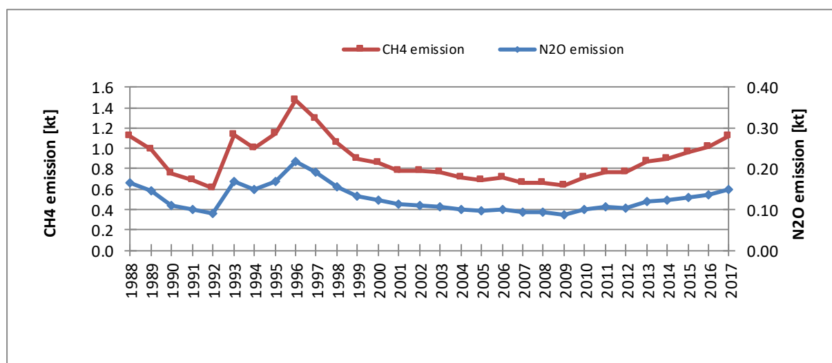
Figure 3.2.7.15. CH 4 and N 2 O emissions from 1.A.2.g category in 1988-2017
