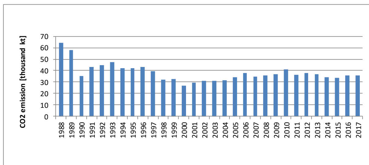
Figure 3.2.9.4. CO 2 emission for 1.A.4.b category in 1988-2017
