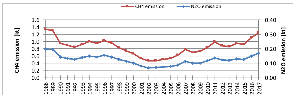
Figure 3.2.7.13. CH 4 and N 2 O emissions from 1.A.2.f category in 1988-2017
