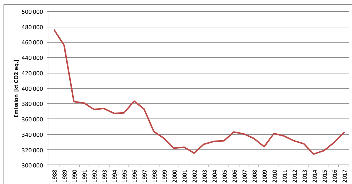
Figure 3.1.1. GHG emission trend in period 1988-2017 in sector Energy
