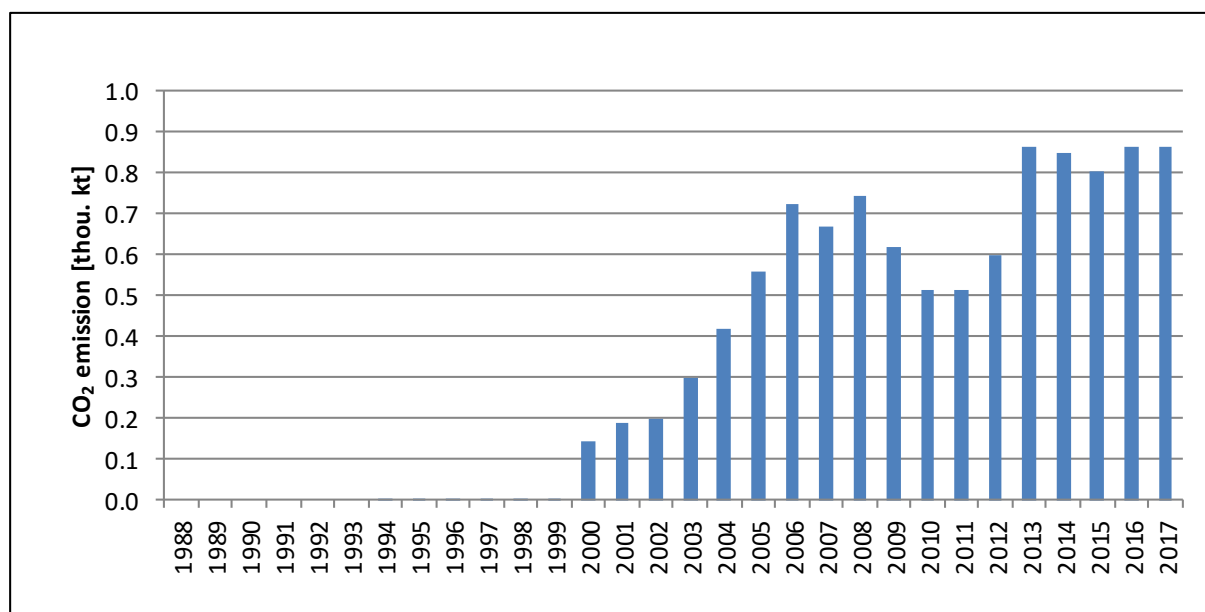
Figure 3.2.8.15. CO 2 emission from Pipelines category in 1988-2017
