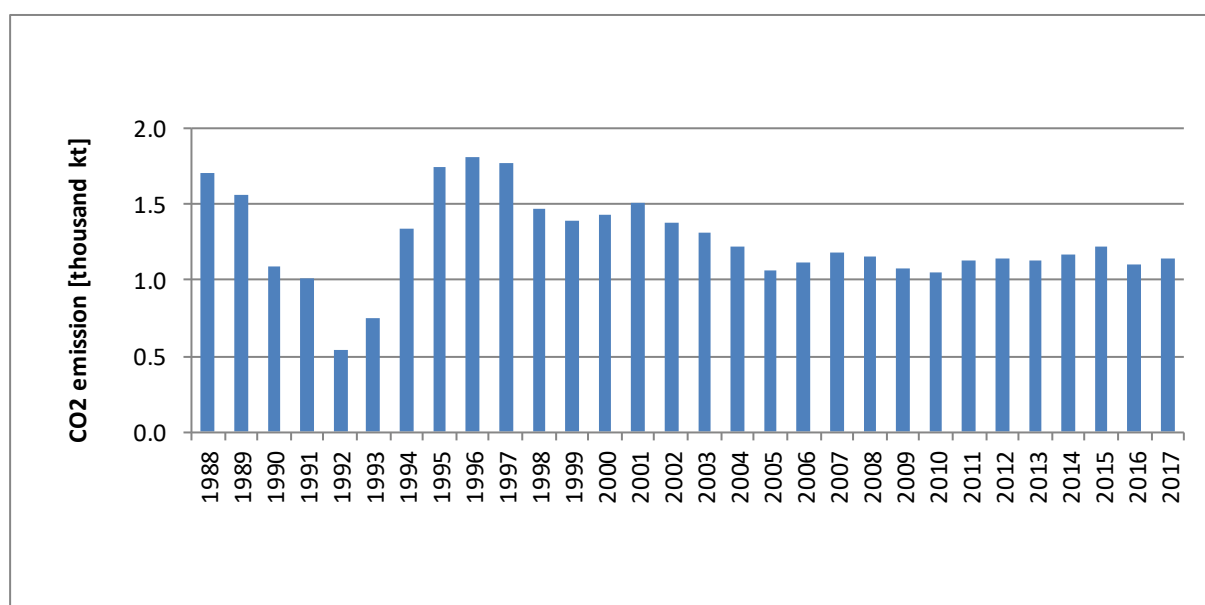
Figure 3.2.7.4. CO 2 emission for 1.A.2.b category in 1988-2017
