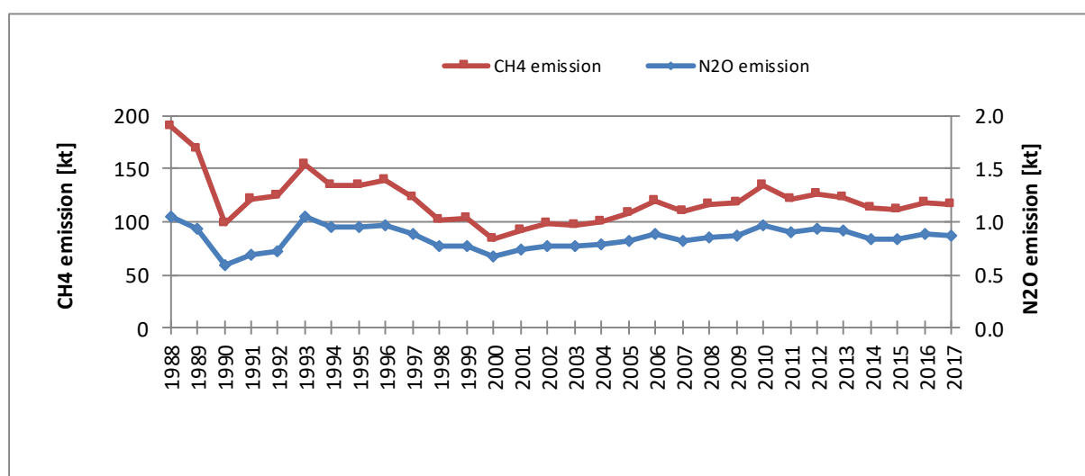
Figure 3.2.9.5. CH 4 and N 2 O emissions for 1.A.4.b category in 1988-2017
