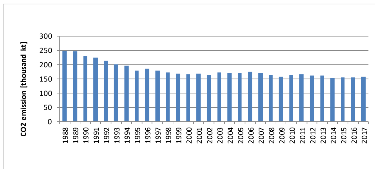
Figure 3.2.6.2. CO 2 emission for 1.A.1.a category in 1988-2017
