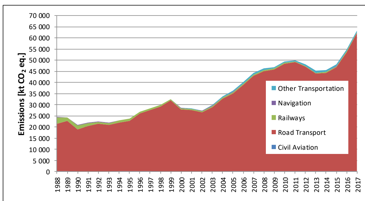
Figure 3.2.8.1. Emissions from transport in years 1988-2017
