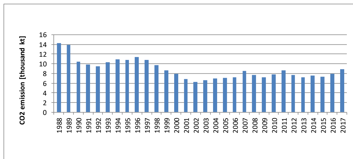
Figure 3.2.7.12. CO 2 emission from 1.A.2.f category in 1988-2017
