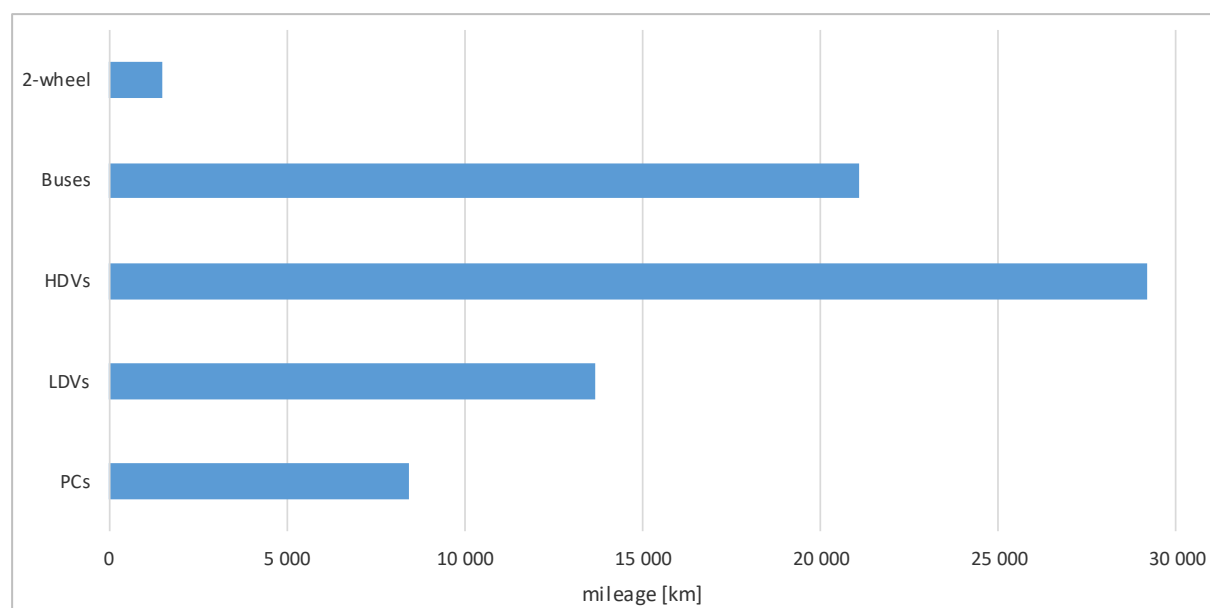
Figure 3.2.8.6. Average annual mileage driven by vehicles in 2017
