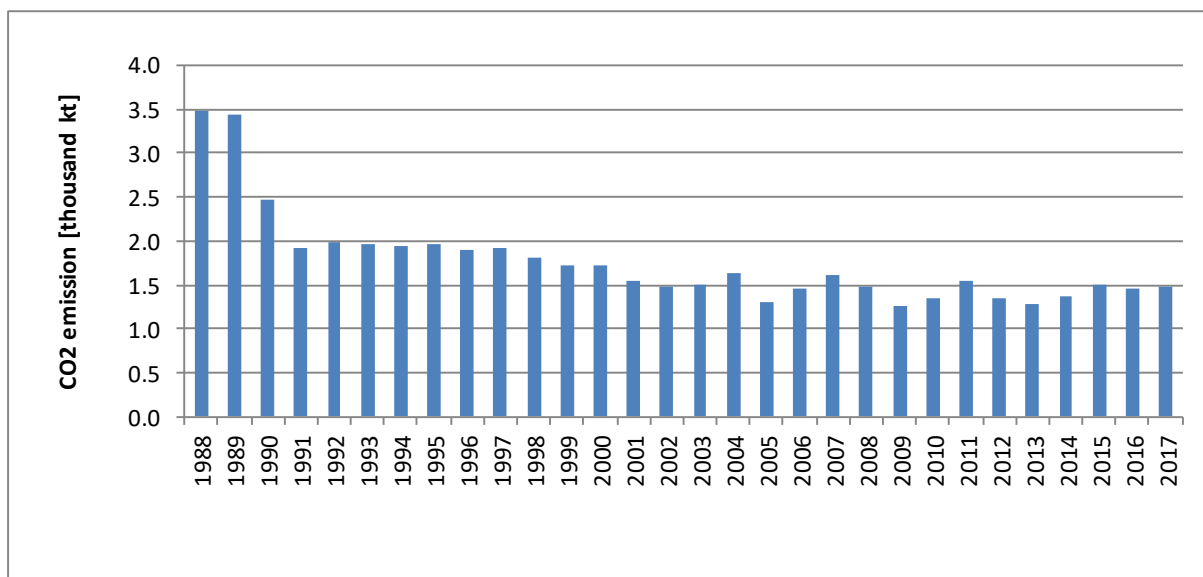
Figure 4.2.5. CO 2 process emission for lime production in 1988-2017
