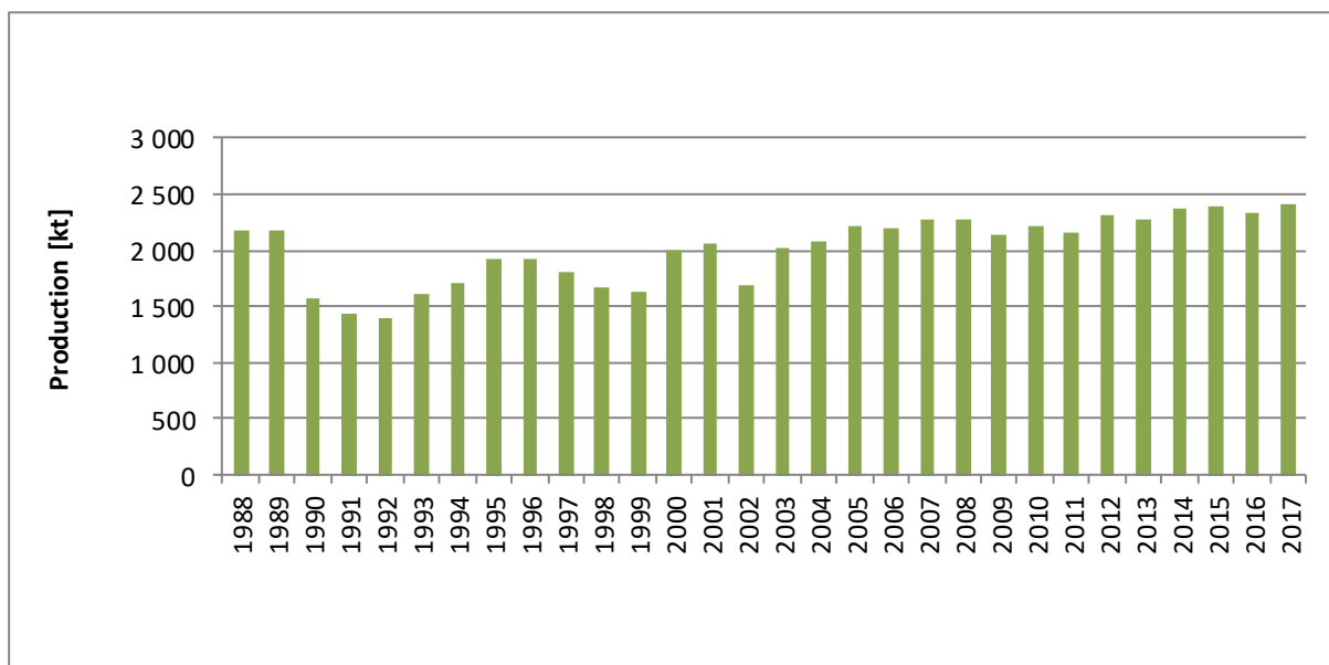
Figure 4.3.4. Production of nitric acid in 1988-2017
