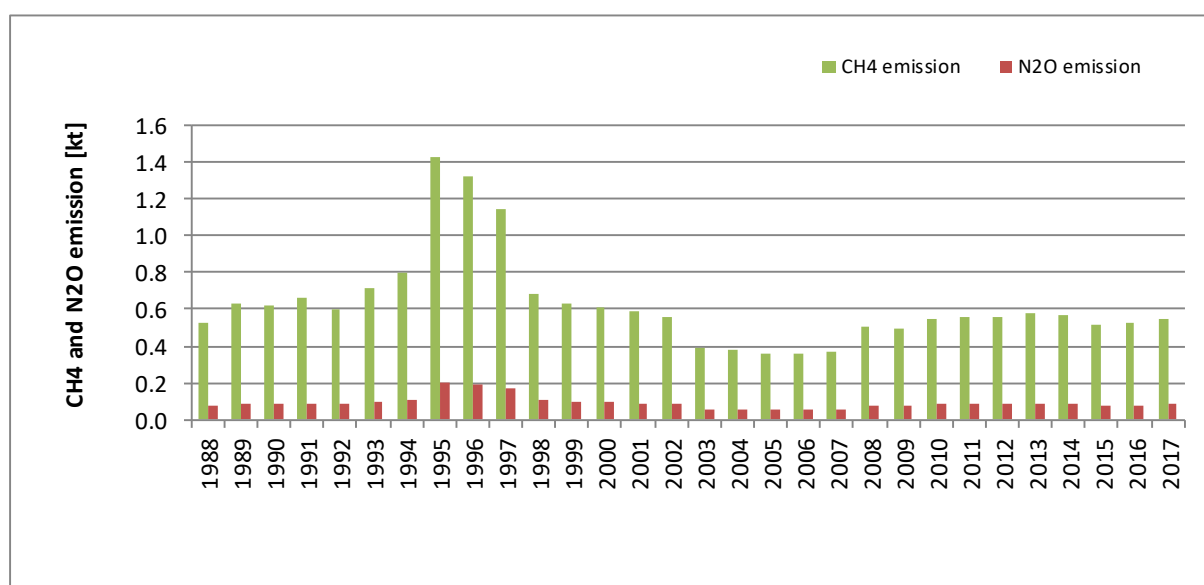
Figure 3.2.7.7. CH 4 and N 2 O emissions for 1.A.2.c category in 1988-2017
