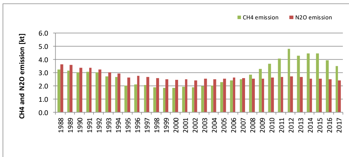
Figure 3.2.6.3. CH 4 and N 2 O emissions for 1.A.1.a category in 1988-2017
