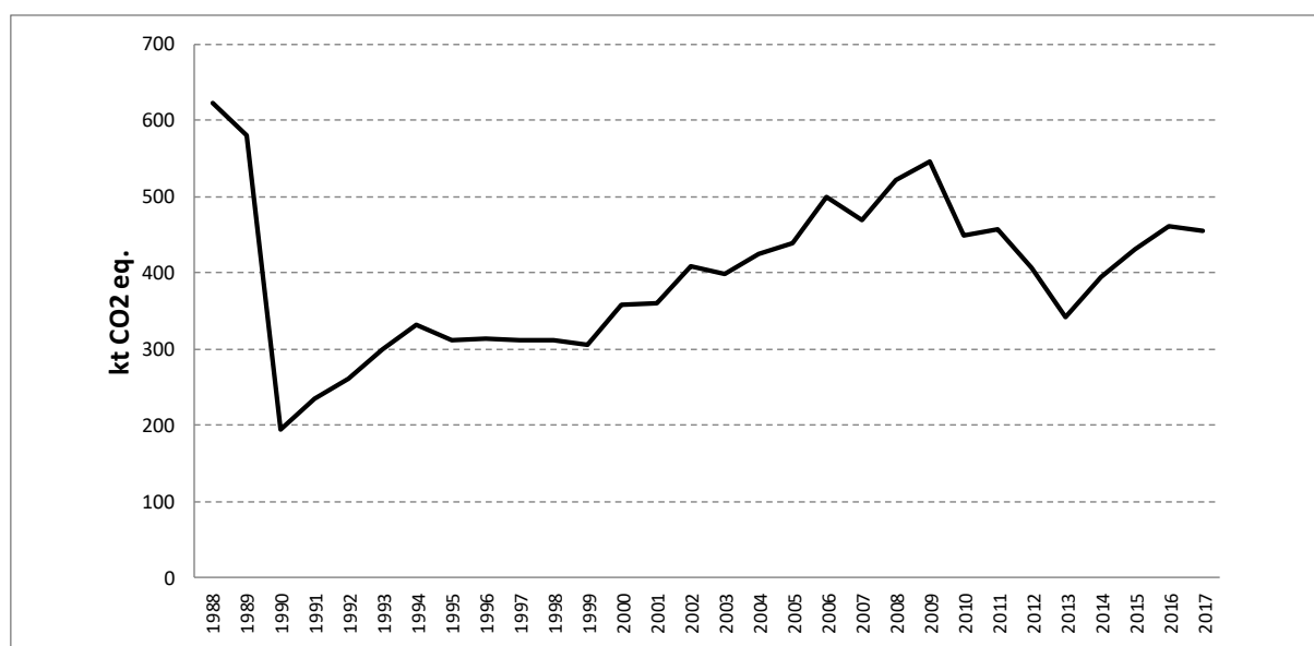
Figure 4.5.4. GHG emission from Solvent and Other Product Use sector in 1988-2017
