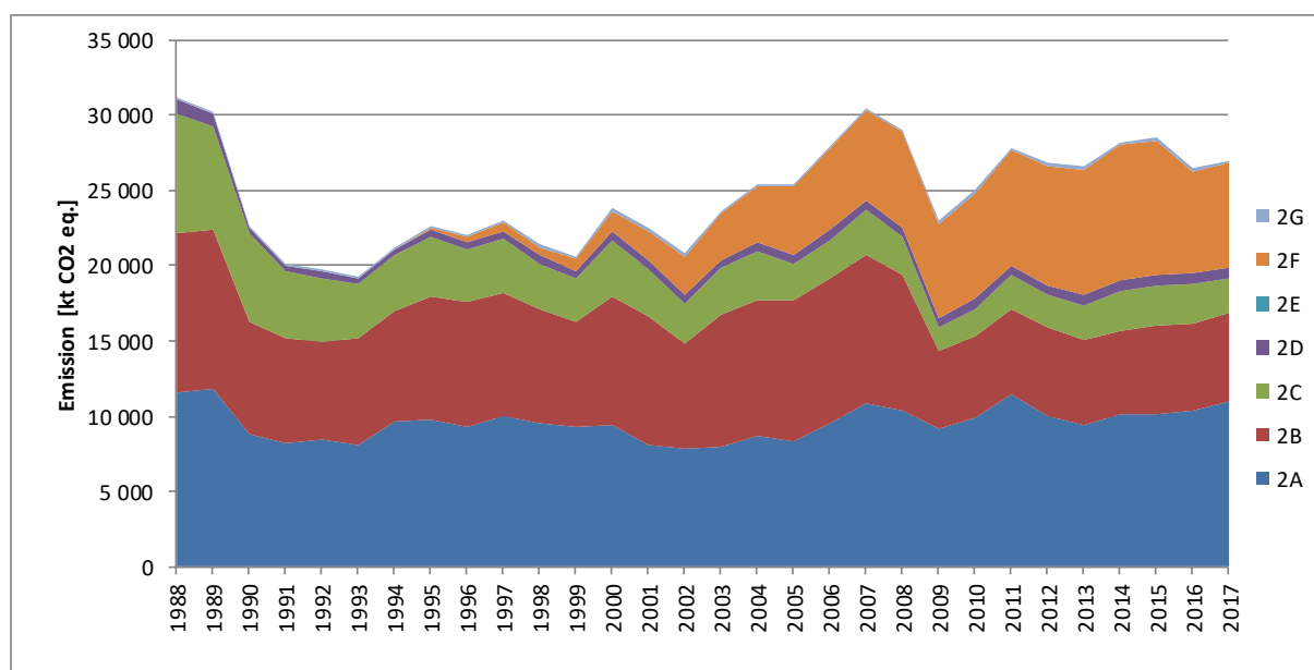
Figure 4.1.2. GHG emissions from Industrial processes and product use in 1988-2017 according to subcategories
