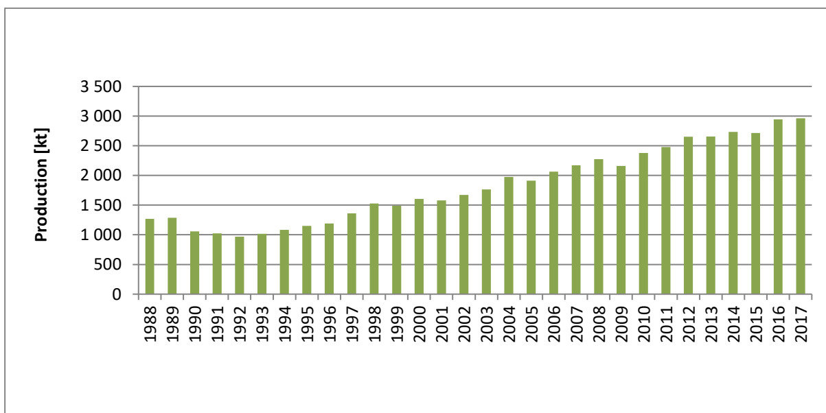
Figure 4.2.6. Glass production in 1988-2017
