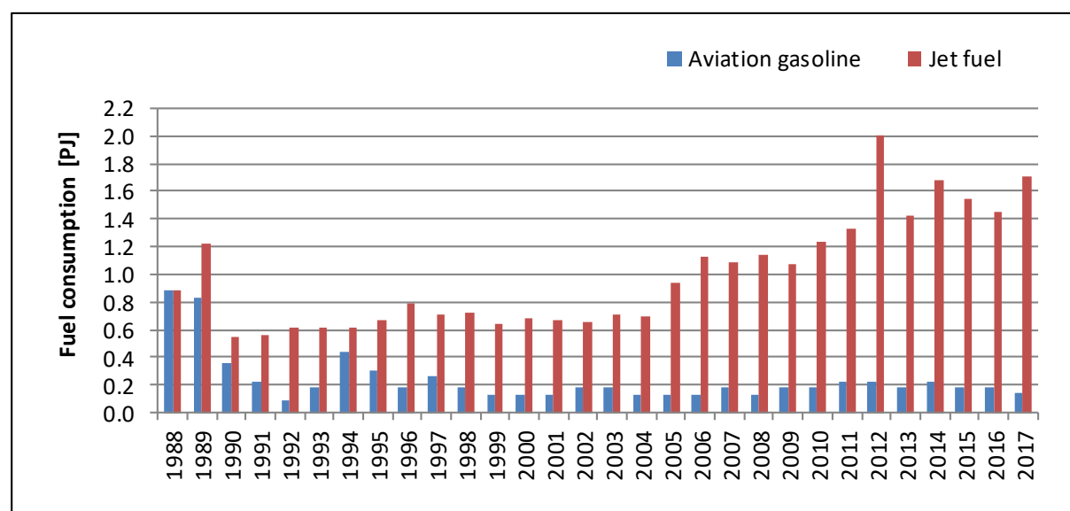
Figure 3.2.8.2. Fuel consumption in 1.A.3.a category for 1988-2017
