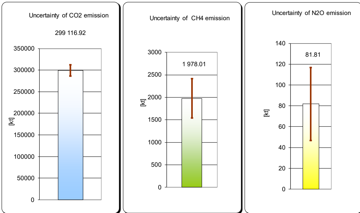
Emission results for 2017 including IPCC 4. LULUCF with uncertainties bars
