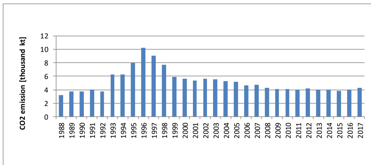
Figure 3.2.7.10. CO 2 emission for 1.A.2.e category in 1988-2017
