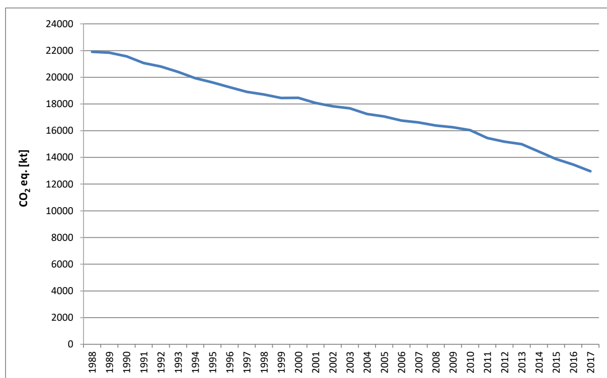
Figure 7.1. GHG emissions from waste sector in 1988-2017
