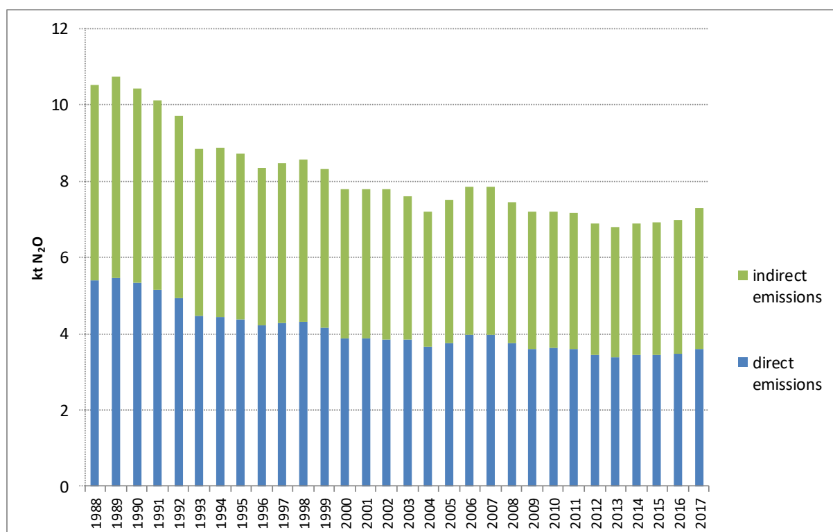
Figure 5.5. Trend of N 2 O emissions (in division for direct and indirect) from manure management
