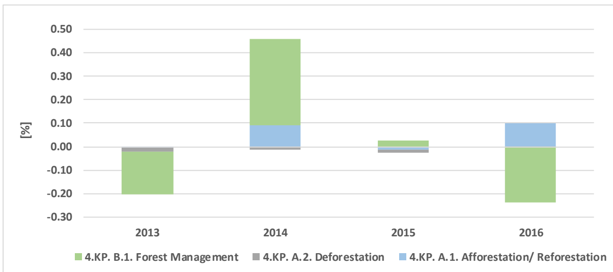
Figure 10.4. Recalculation of CO 2 for 2013-2016 for KP-LULUCF activities made in CRF 2019 comparing to CRF 2018
