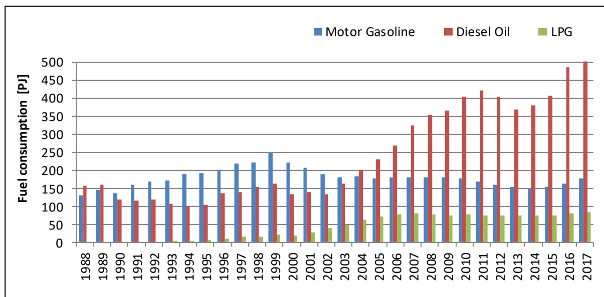
Figure 3.2.8.5. Fuel consumption in 1.A.3.b category for 1988-2017
