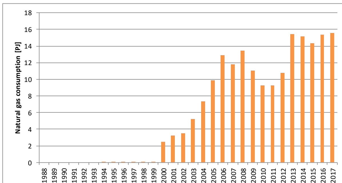
Figure 3.1.8.14. Natural gas consumption in Pipelines transport category for 1988-2017
