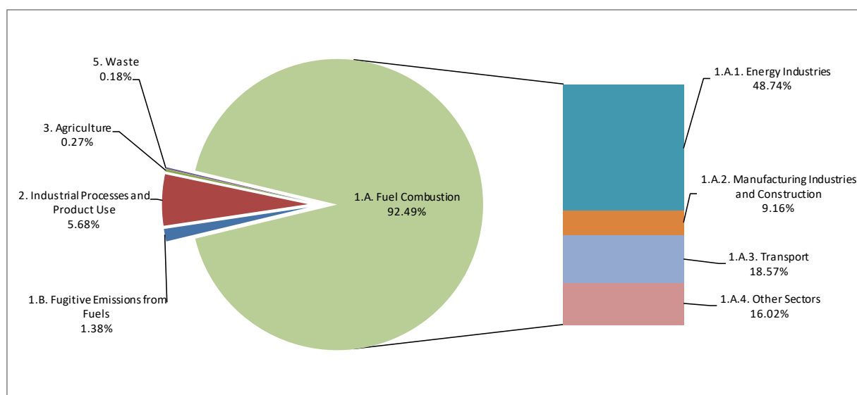
Figure 2.3. Carbon dioxide emission (excluding category 4) in 2017 by sector
