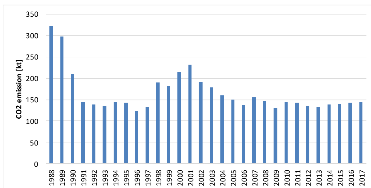
Figure 4.5.2. CO 2 emissions from non-energy use of lubricants in years 1988-2017
