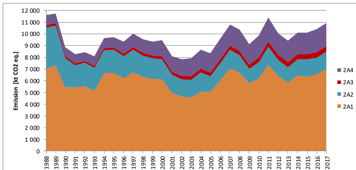
Figure 4.2.1. Emissions from Mineral industry sector in years 1988-2017 according to subcategories
