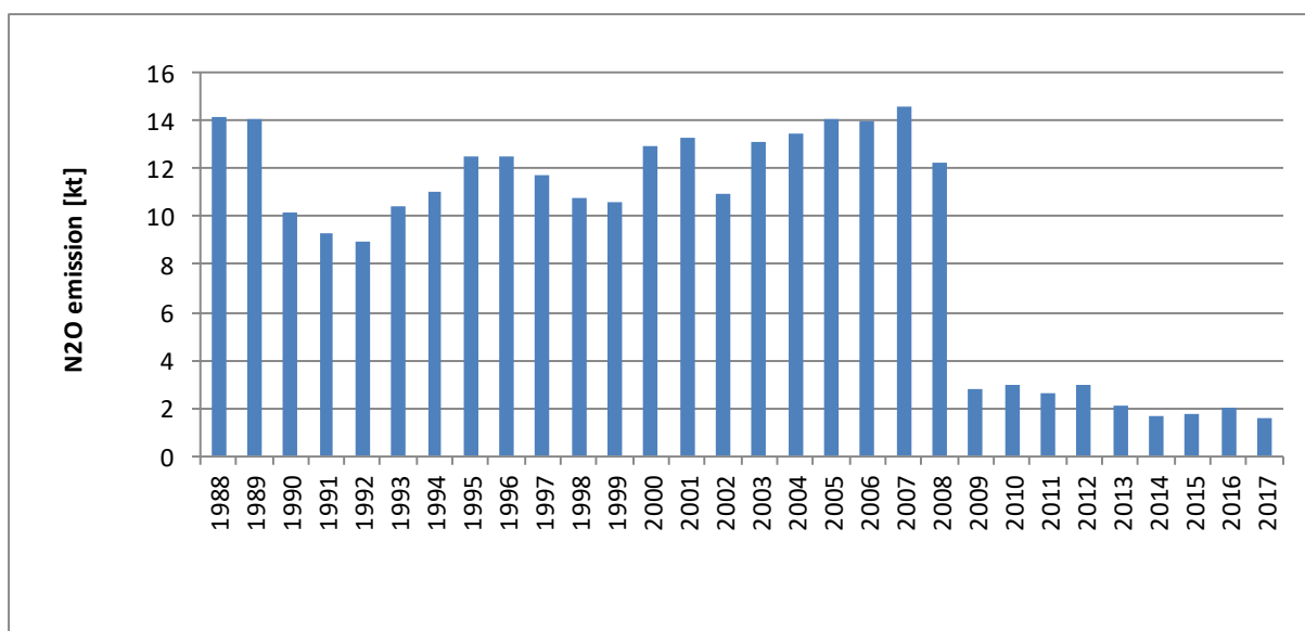
Figure 4.3.5. N 2 O process emission for nitric acid production in 1988-2017
