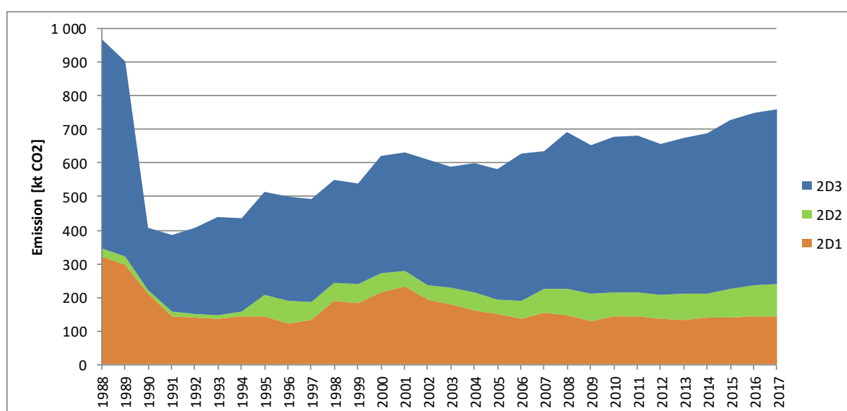
Figure 4.5.1. Emissions from Non Energy Product from Fuels and Solvent Use sector in years 1988-2017 according to subcategories
