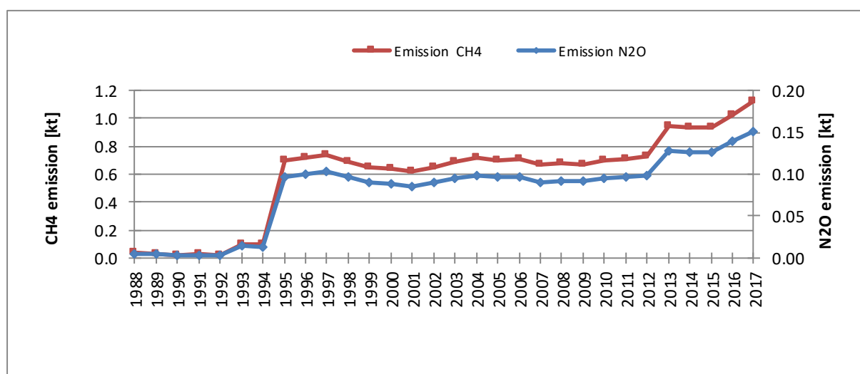
Figure 3.2.7.9. CH 4 and N 2 O emissions for 1.A.2.d category in 1988-2017
