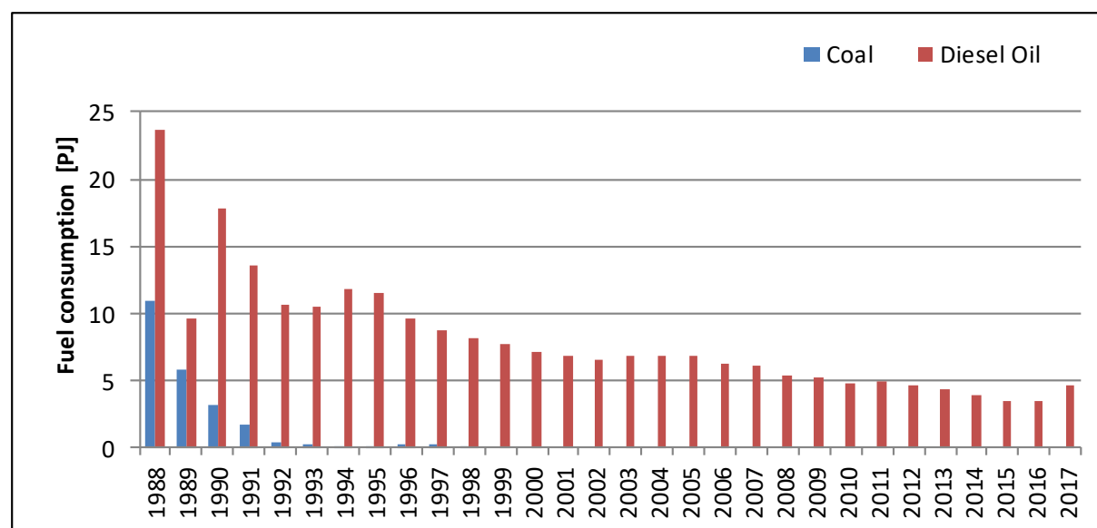
Figure 3.2.8.8. Fuel consumption in 1.A.3.c category for 1988-2017
