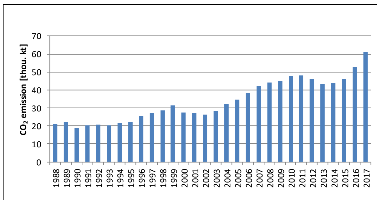
Figure 3.2.8.6. CO 2 emission for 1.A.3.b category in 1988-2017
