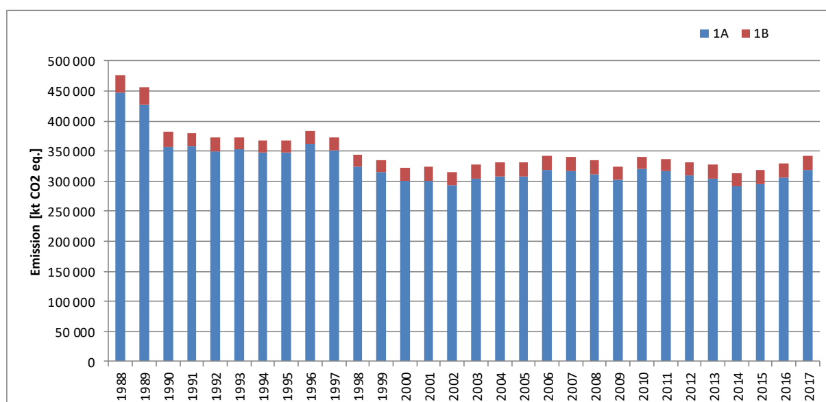
Figure 3.1.2. GHG emission trend in period 1988-2017 in subsectors 1.A and 1.B
