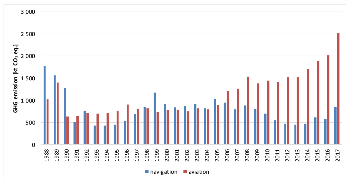
Figure 3.2.1. GHG emissions from international navigation and aviation bunker in period 1988-2017
