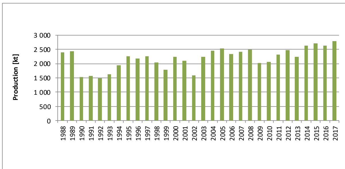
Figure 4.3.3. Production of ammonia in 1988-2017
