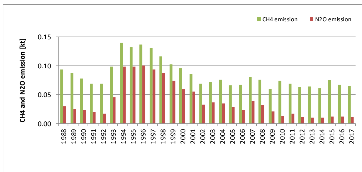
Figure 3.2.6.7. CH 4 and N 2 O emissions for 1.A.1.c category in 1988-2017
