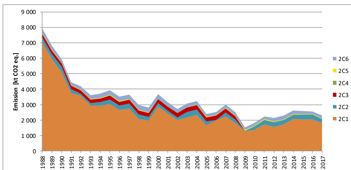
Figure 4.4.1. Emissions from Metal industry sector in years 1988-2017 according to subcategories
