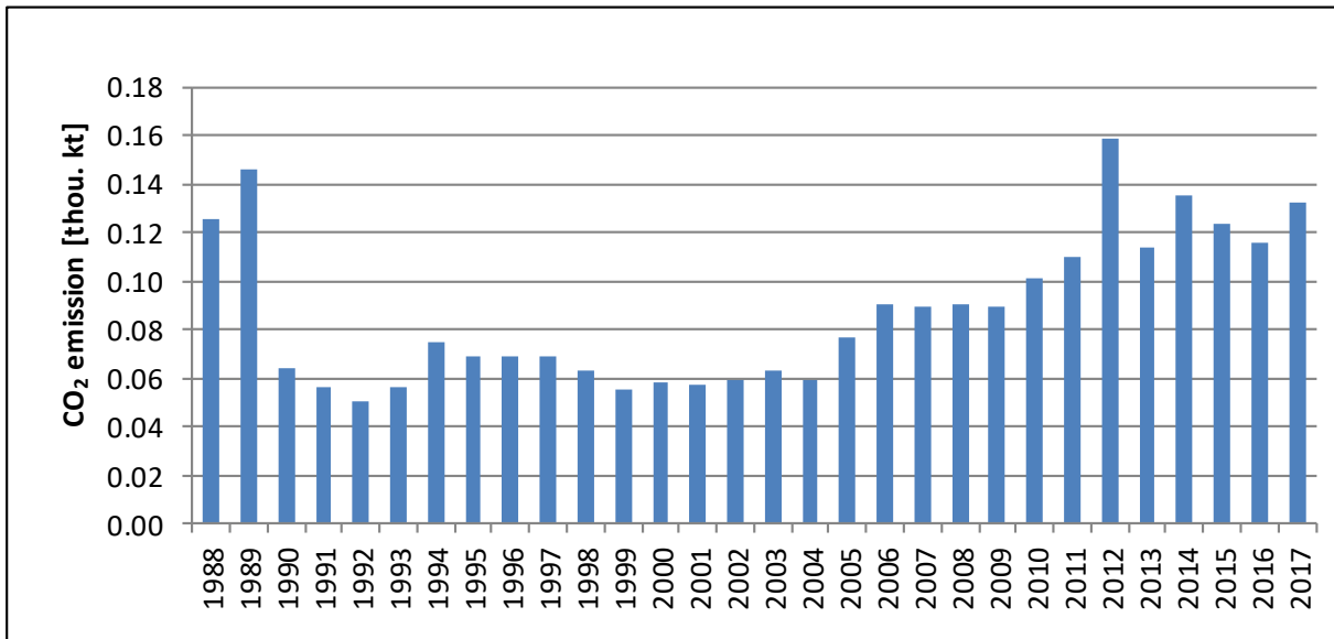
Figure 3.2.8.3. CO 2 emission for 1.A.3.a category in 1988-2017
