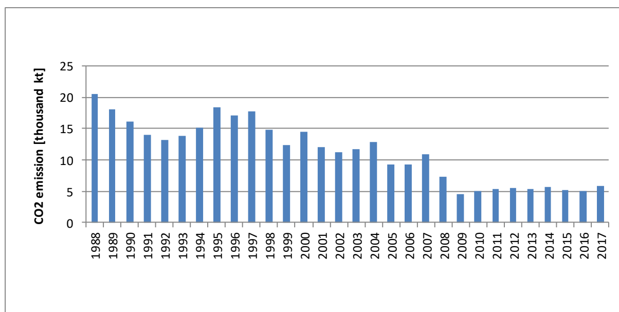
Figure 3.2.7.2. CO 2 emission for 1.A.2.a category in 1988-2017
