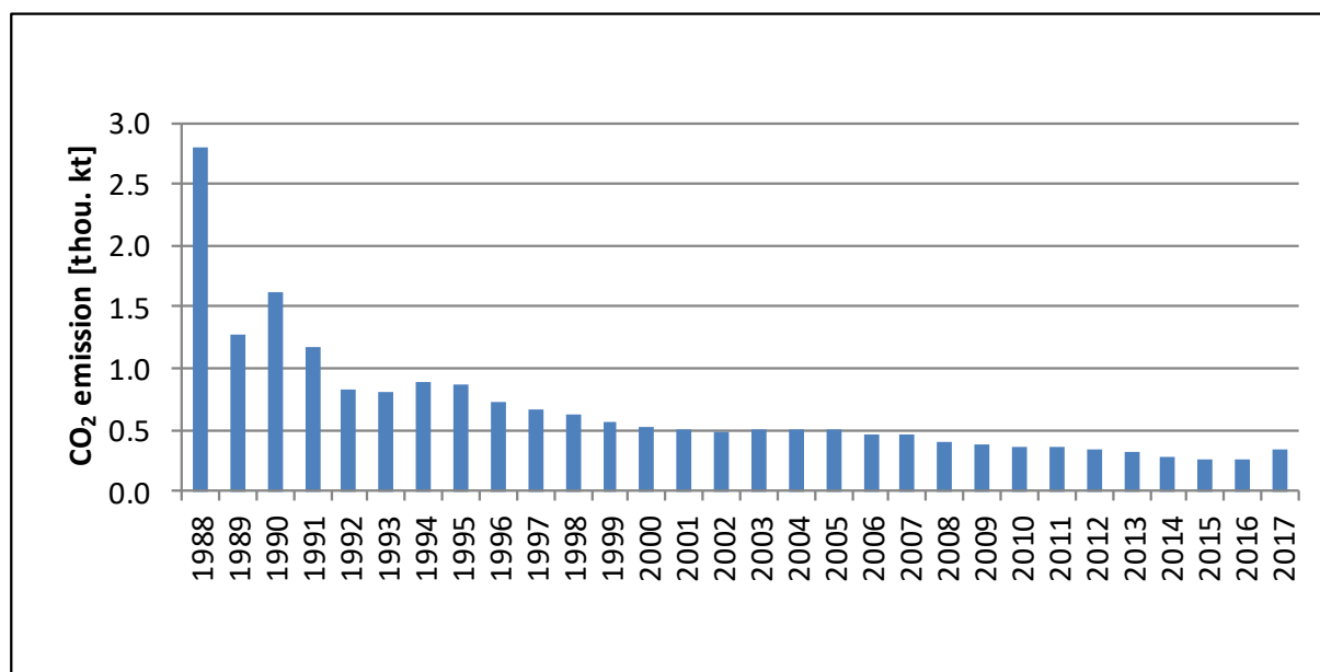
Figure 3.2.8.9. CO 2 emission for 1.A.3.c category in 1988-2017
