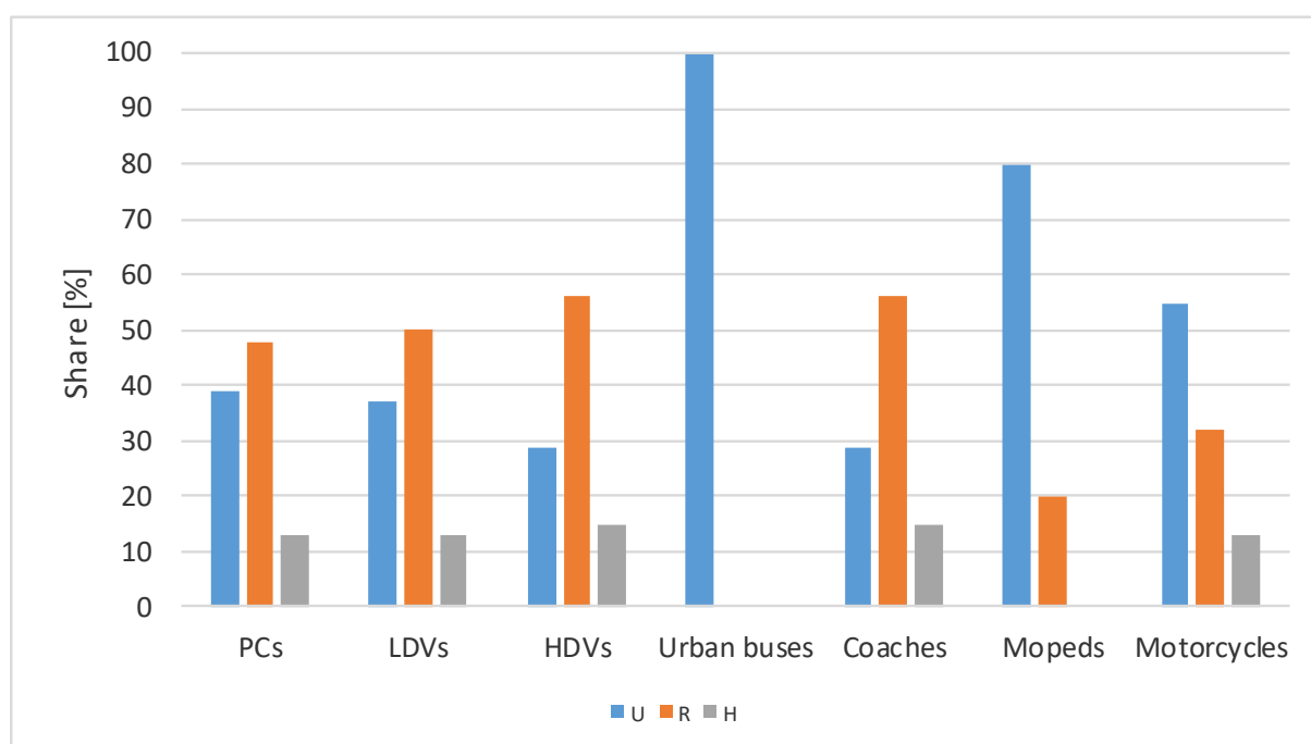
Figure 3.2.8.7. Mileage share per road class (urban, rural and highways) in 2017
