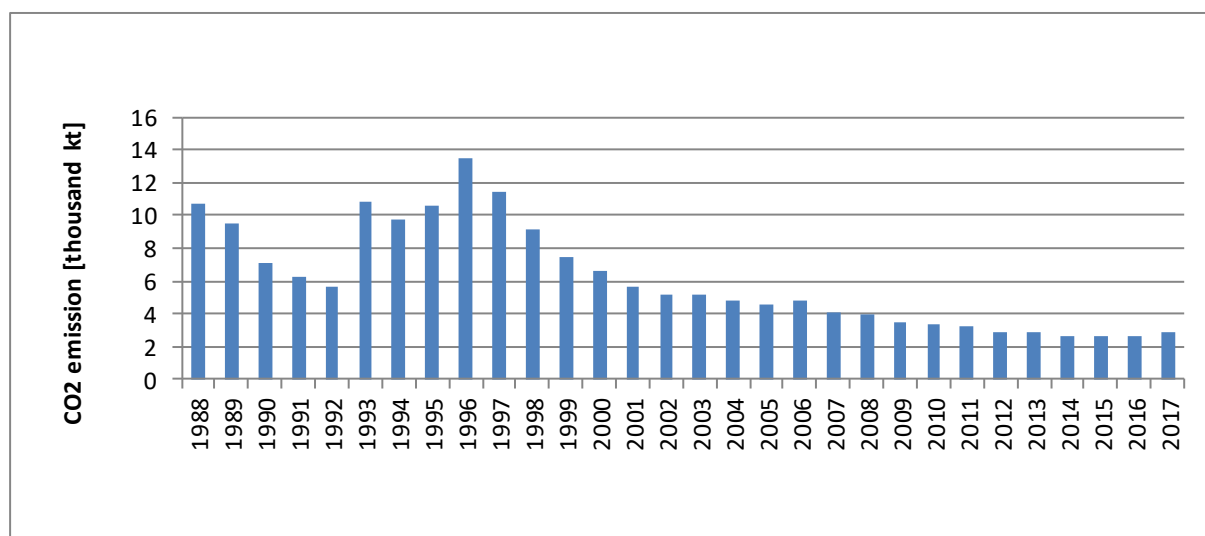
Figure 3.2.7.14. CO 2 emission from 1.A.2.g category in 1988-2017
