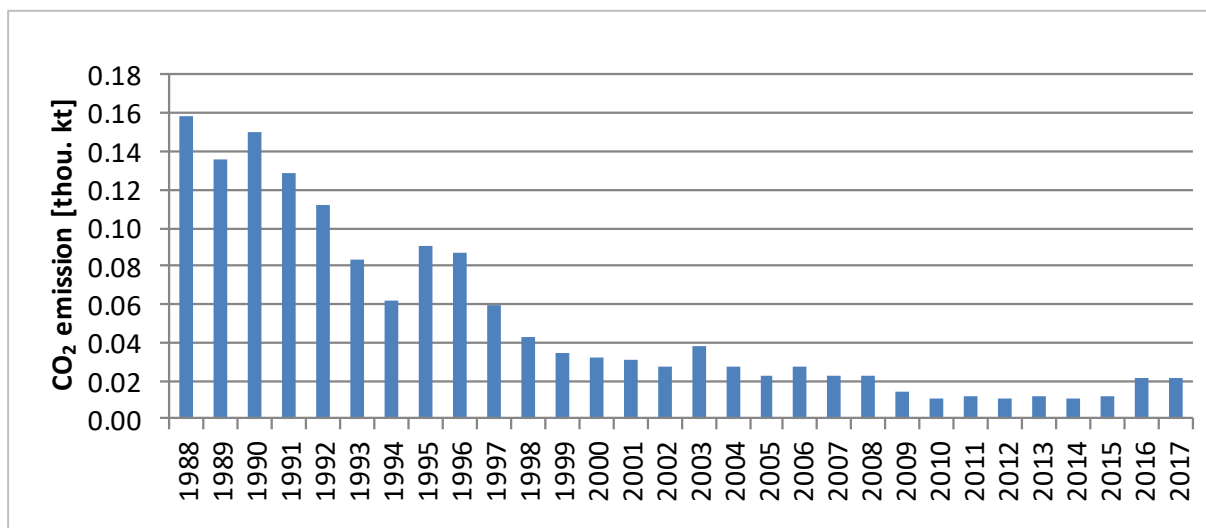
Figure 3.2.8.12. CO 2 emission for 1.A.3.d category in 1988-2017
