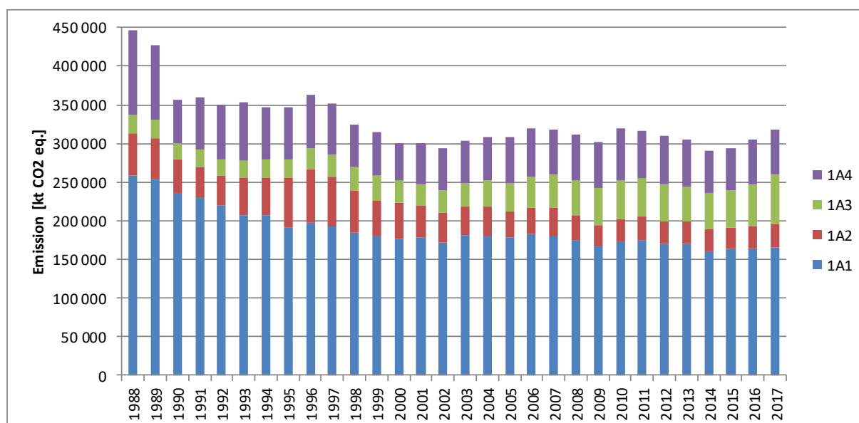
Figure 3.1.3. GHG emissions from fuel combustion in 1988-2017 according to subcategories
