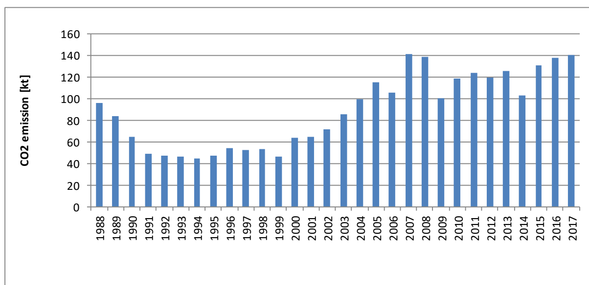
Figure 4.2.9. CO 2 process emission from ceramics in 1988-2017
