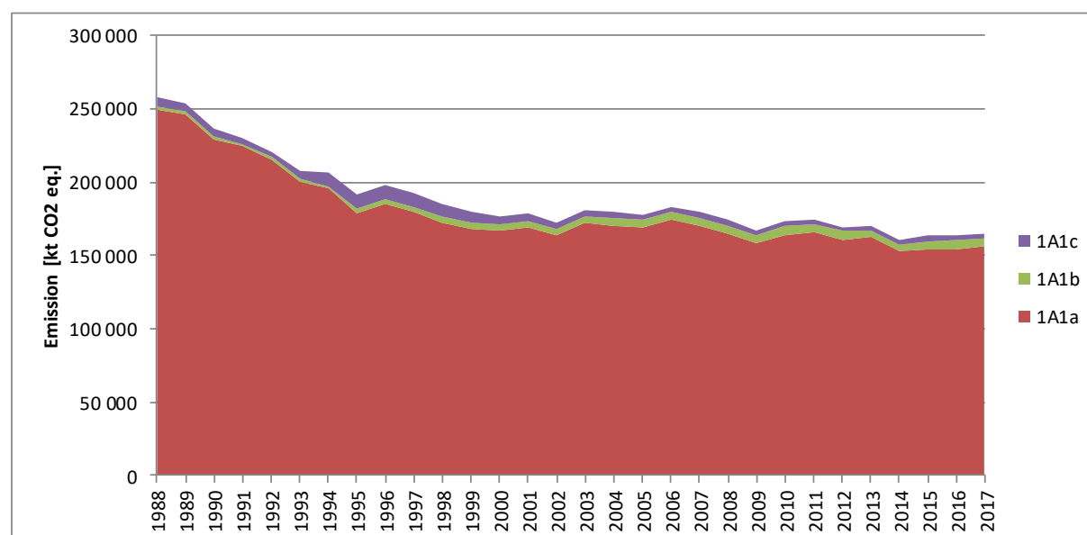
Figure 3.2.6.1. GHG emissions from Energy Industries in years 1988-2017 according to subcategories
