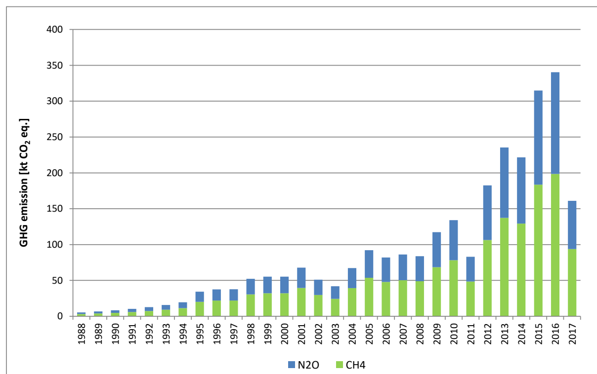
Figure 7.6. GHG emission from 5.B subsector
