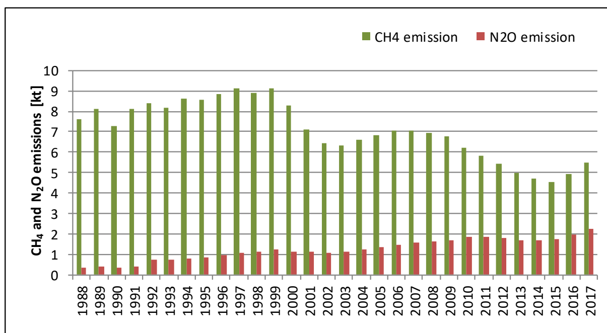
Figure 3.2.8.7. CH 4 and N 2 O emissions for 1.A.3.b category in 1988-2017
