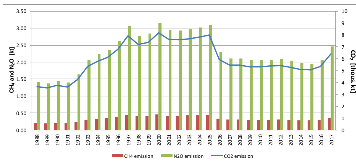
Figure 3.2.8.18. GHG emission in 1988-2017 in subcategory 1.A.4.c.ii
