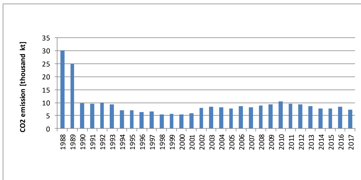
Figure 3.2.9.2. CO 2 emission for 1.A.4.a category in 1988-2017
