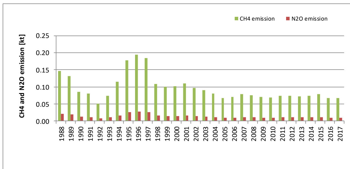
Figure 3.2.7.5. CH 4 and N 2 O emissions for 1.A.2.b category in 1988-2017
